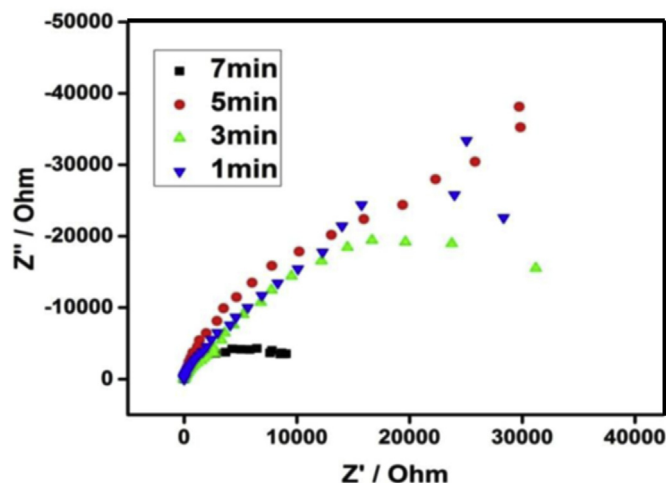
Fig. 7 – EIS for 1, 3, 5 and 7 min cathodized defect rich titania nanostructure samples.
