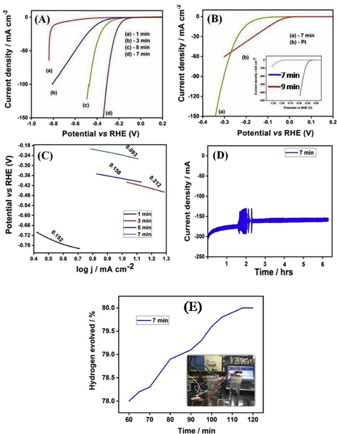
Fig. 8 – A. Polarization results for (a) 1, (b) 3, (c) 5 and (d) 7 min cathodized defect rich titania nanostructure samples in 1 M \text{H}_2\text{SO}_4 aqueous electrolyte with scan rate of 0.010 \text{ V s}^{-1} for HER. B. HER activity studies for a) 7 min cathodized defect rich titania nanostructure sample and b) Pt, and insert image show the HER activity of 7 and 9 min sample. C. Tafel slope for 1, 3, 5 and 7 min cathodized defect rich titania nanostructure samples. D. Stability test for 7 min cathodized defect rich titania nanostructure sample. E. The collection of hydrogen gas (in percentage) was investigated using hydrogen sensor for 7 min defect rich titania nanostructure.
