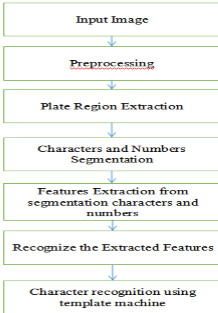
Fig 4.1 System Architecture
