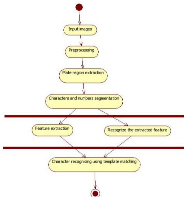
Fig 4.4 Activity diagram
