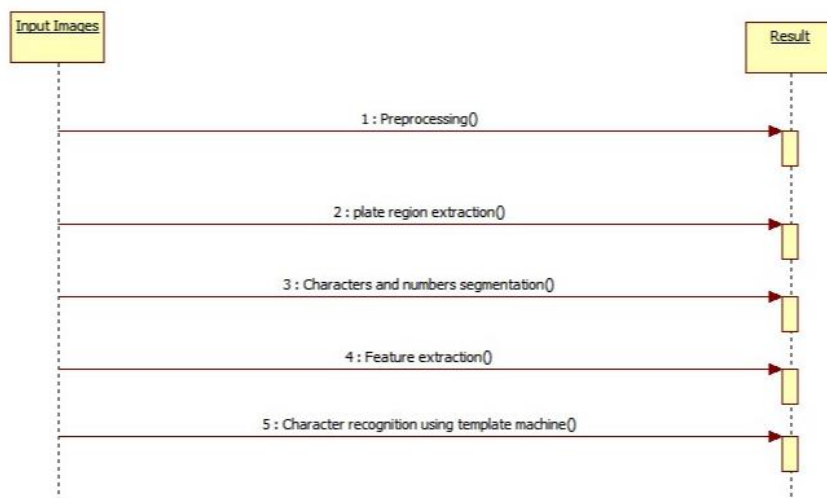
Fig 4.3 Sequence diagram
