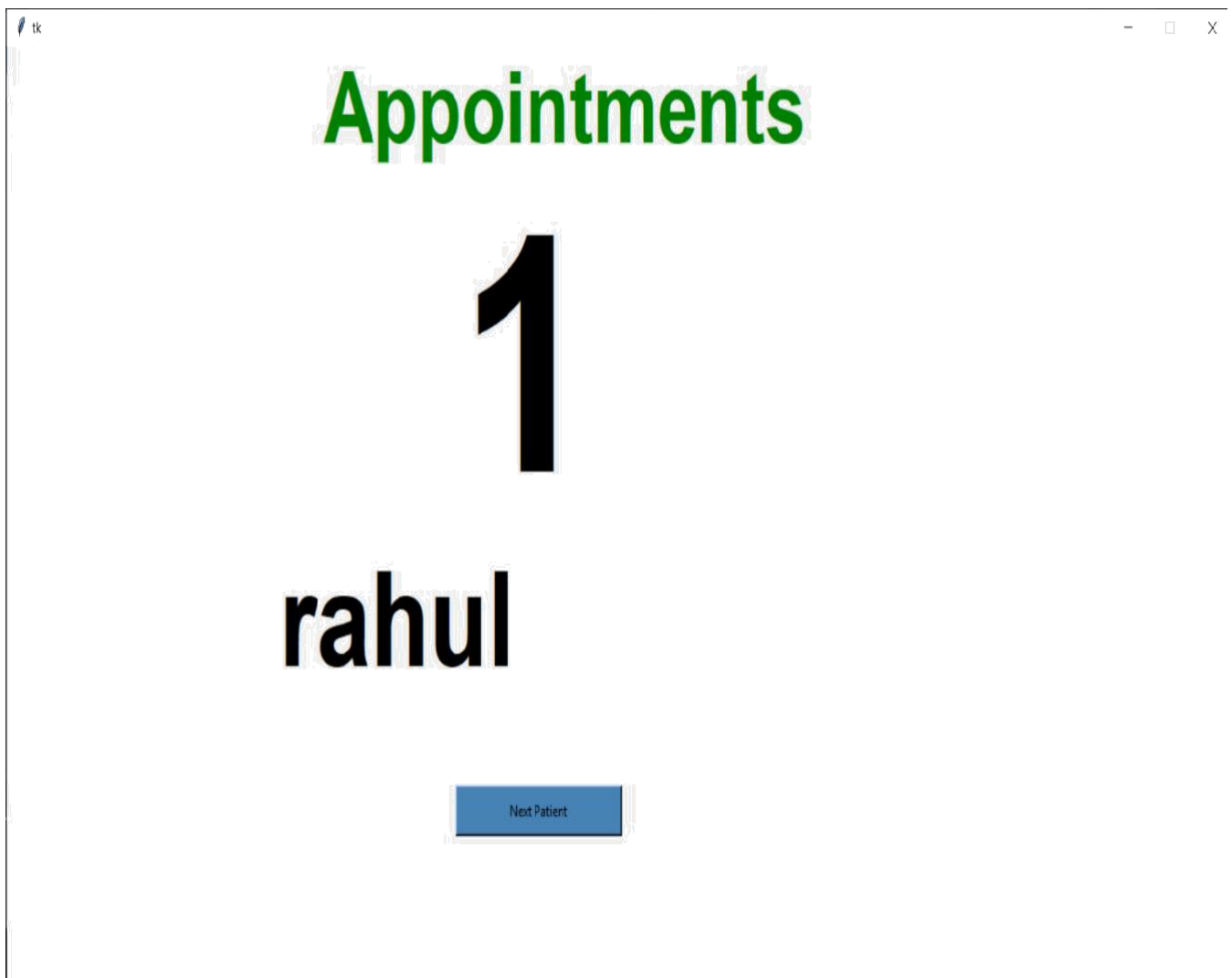
Fig 5.5 Displaying Appointment
