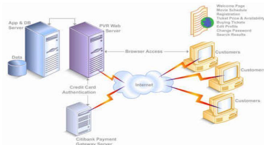
Fig 2.1 Internet booking
