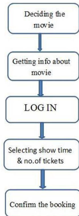
Fig 3.3.2 Activity Diagram 1
