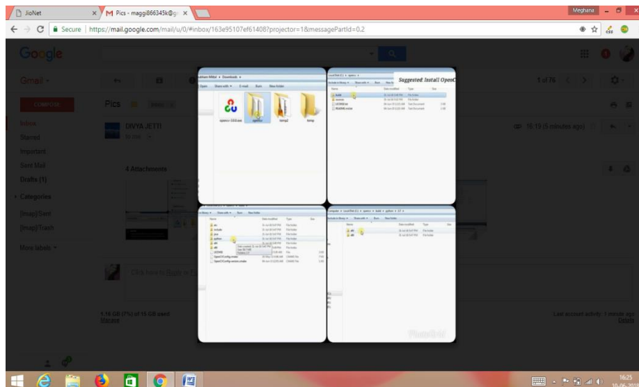
Fig 4.4 Package Installation
