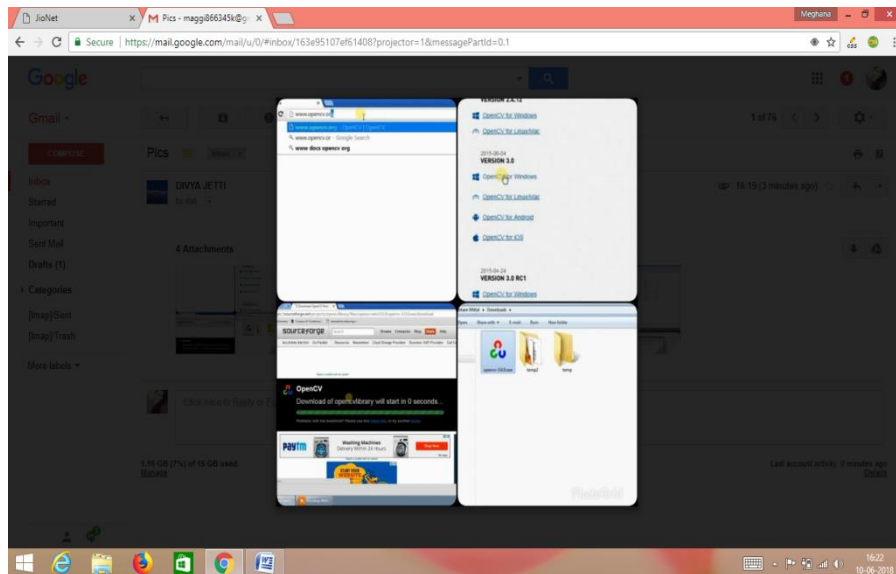
Fig 4.2 Opencv Downloading
