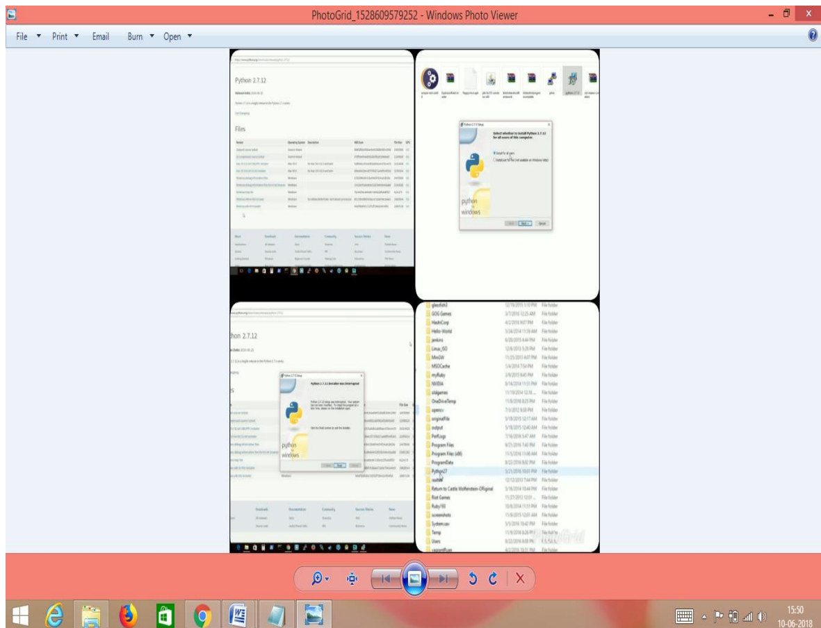
Fig 4.1 Python Installation
