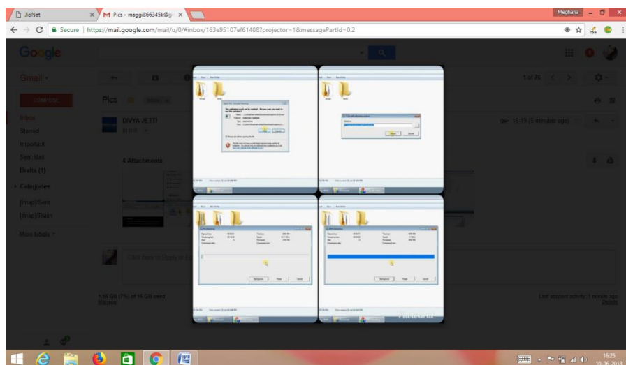
Fig 4.3 Opencv Installation
