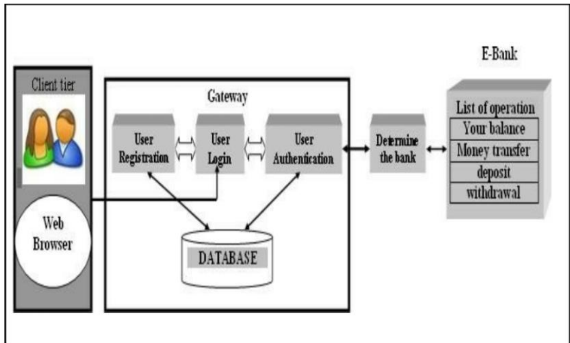
Fig 3.3 Architecture of the Implemented System
