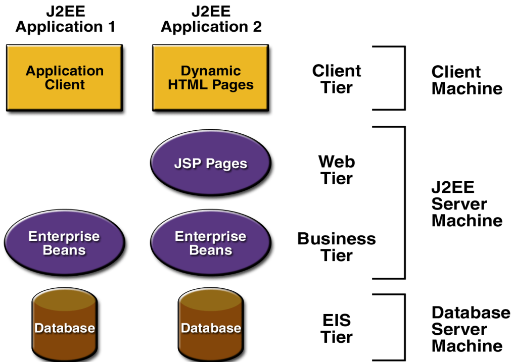
Figure 1-1 Multitiered Applications
