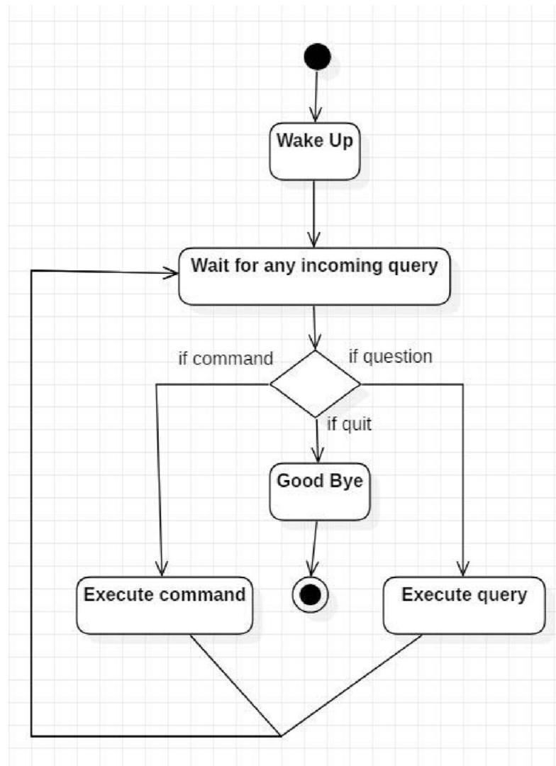
Fig 4.2.2 Activity Diagram
