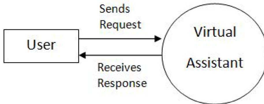
Fig 4.2.6.1 DFD Level 0
