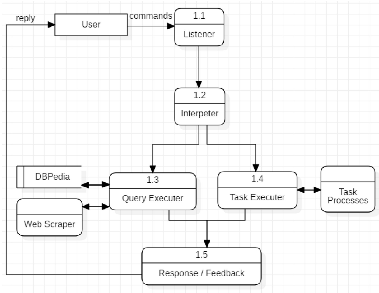
Data Flow in Assistance
