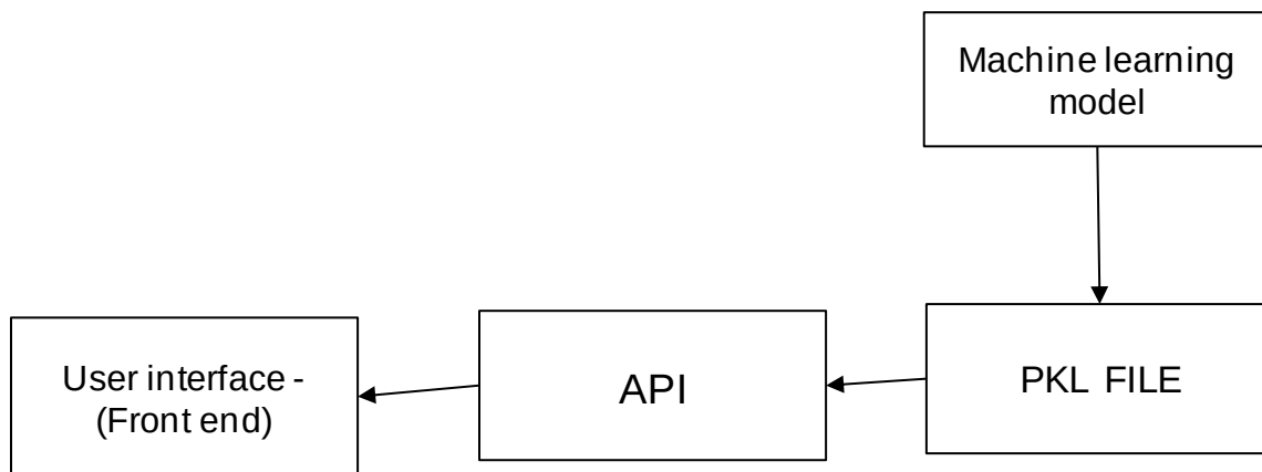
Fig 4.15 Web application Model
