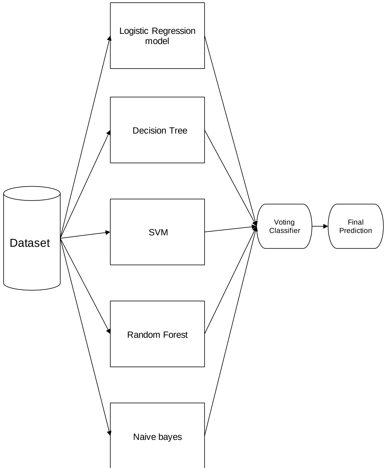
Fig 4.13 Hybrid Ensemble Model
