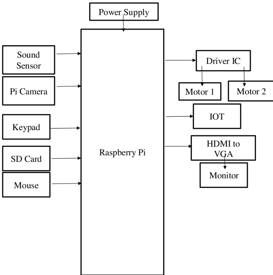
Fig: 3.3 : Block Diagram of proposed System
