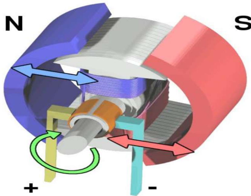
Fig : 4.1.4b DC motor internal view
