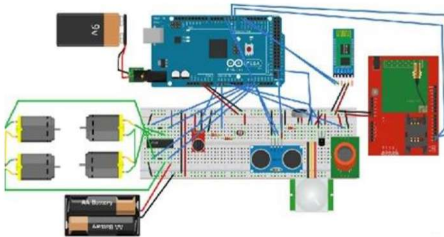
Fig : 2a : Demonstration of robot using android application
