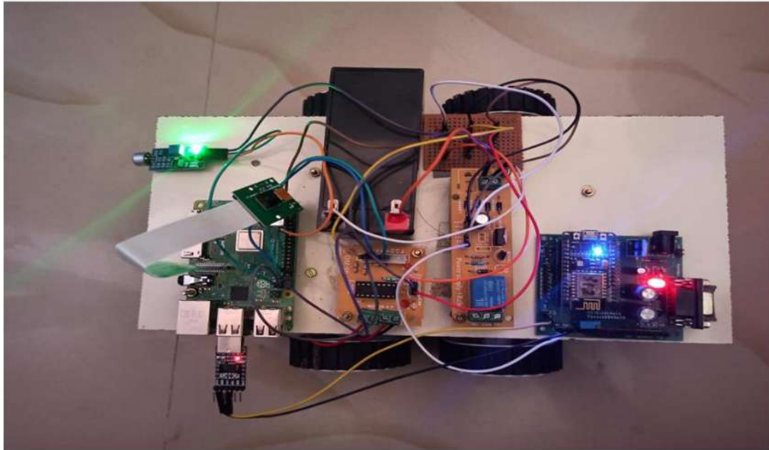
Fig:5.2 : Working of Patrolling Robot
