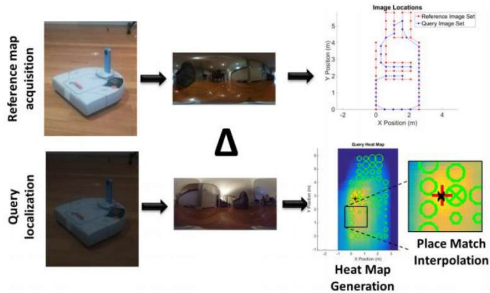
Fig : 2b : 2D-visual robotic system architecture
