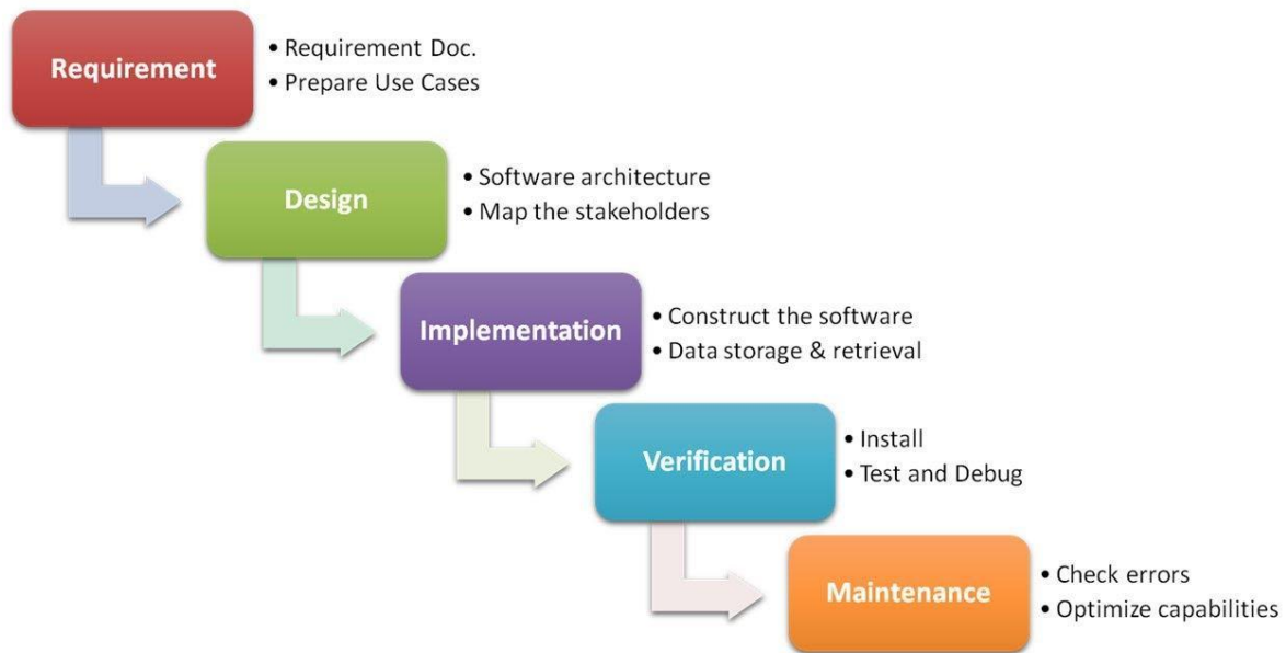
FIG.3.1 WATERFALL MODEL
