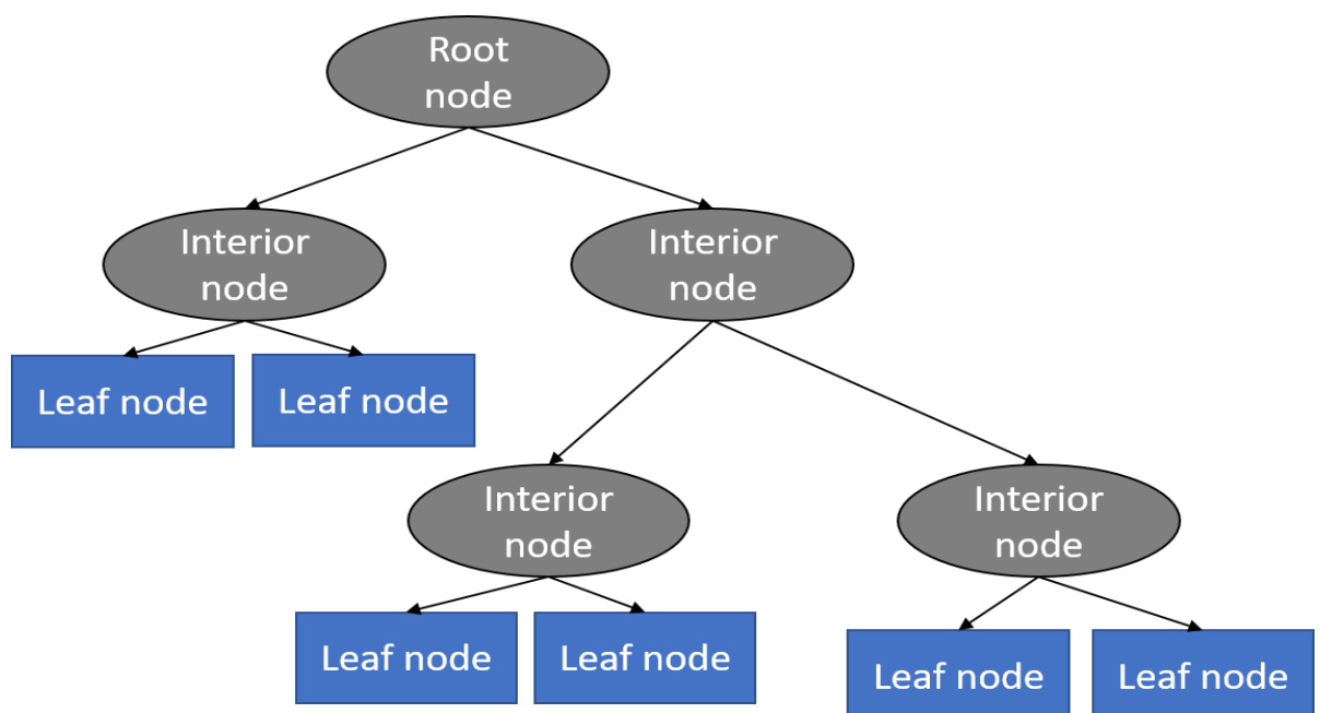
Fig 3.2. Decision Tree
