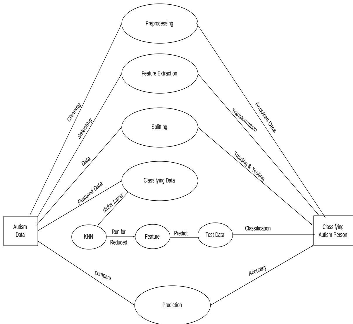
Fig 6.6 : Data Flow Diagram Level 2 for Classifying Data
