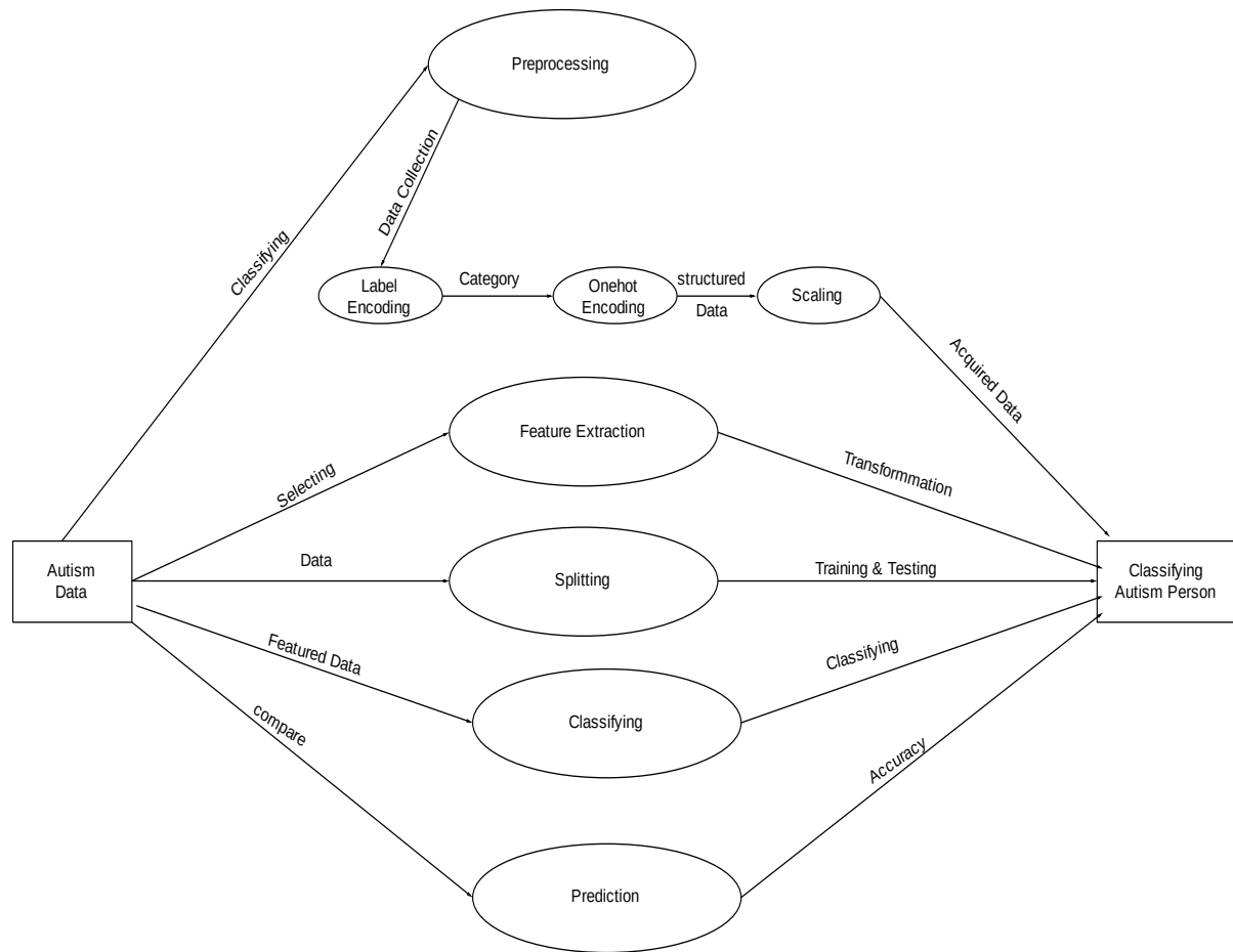
Fig 4.3 :Data Flow Diagram Level 1 for Pre-processing
