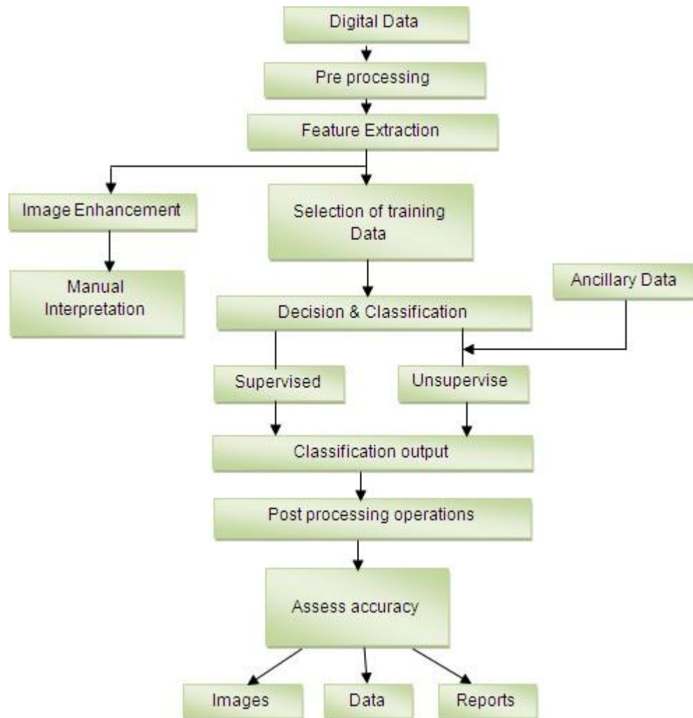
Fig 4.2 Detailing on Image Processing
