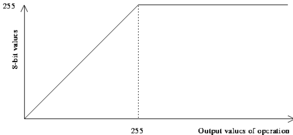
Fig 4.12: Mapping function for saturating an 8-bit image.
