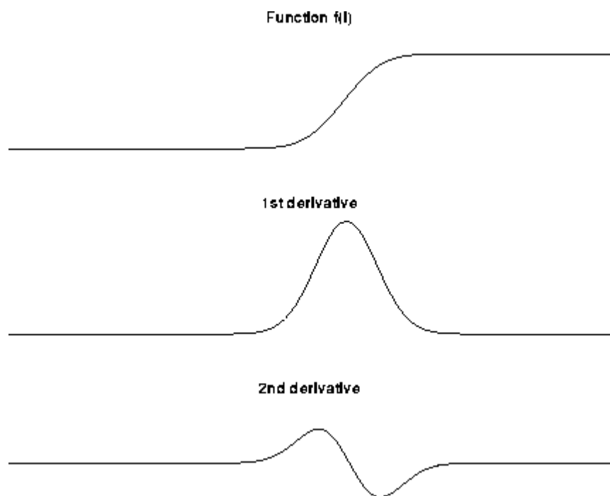
Fig 4.5: 1st and 2nd derivative of an edge illustrated in one dimension.
