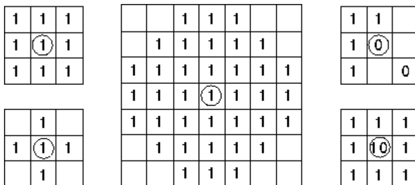
Fig 4.10: Some example structuring elements.
