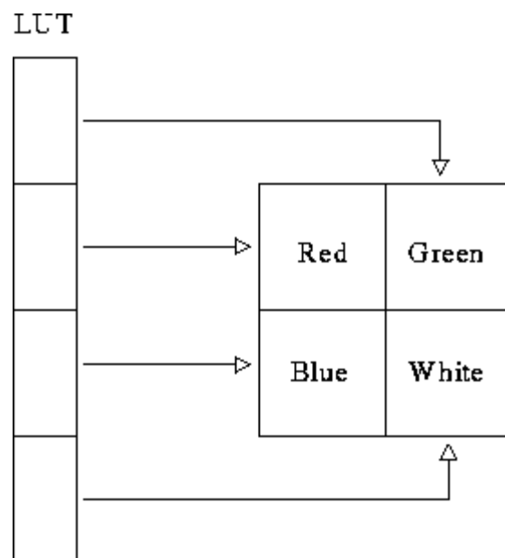
Fig 4.3: A 2×2 pixel area displaying one composite color
