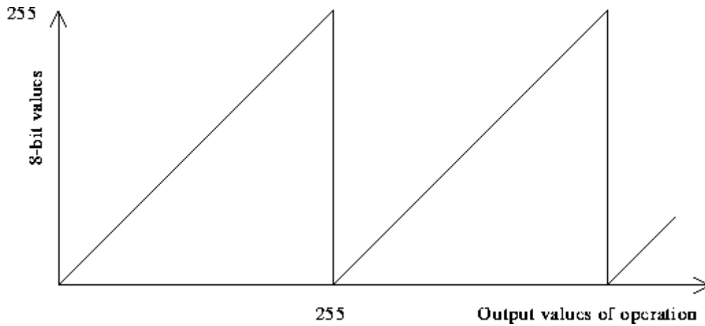
Fig 4.11: Mapping function for wrapping the pixel values of an 8-bit image.
