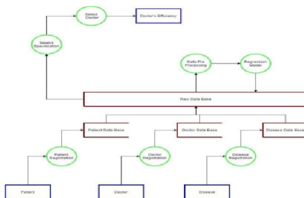
Figure 4.2: Data Flow Diagram
