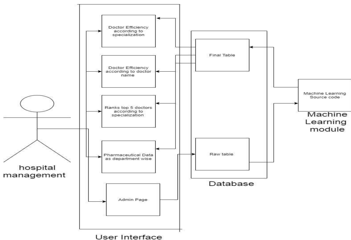
Figure 4.4.2: UML Diagram
