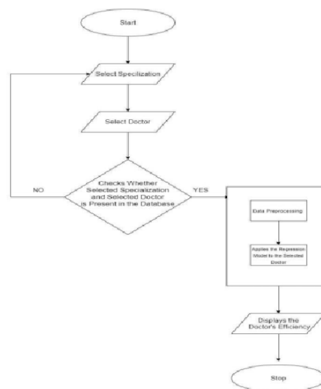
Figure 4.3: Flow Chart
