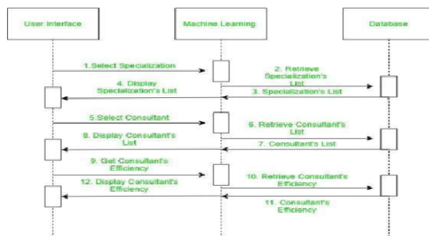
Figure 4.5: Sequence Diagram
