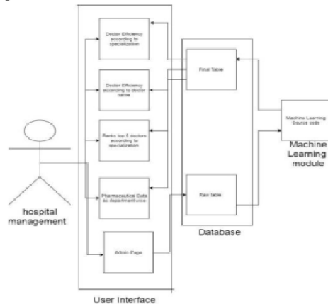
Figure 4.1: UML Diagram
