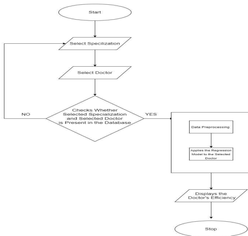
Figure 4.4.3: Flow Chart
