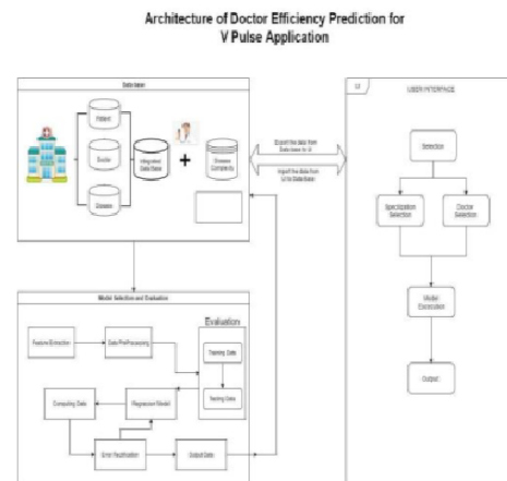
Figure 4.2: Architecture Diagram
