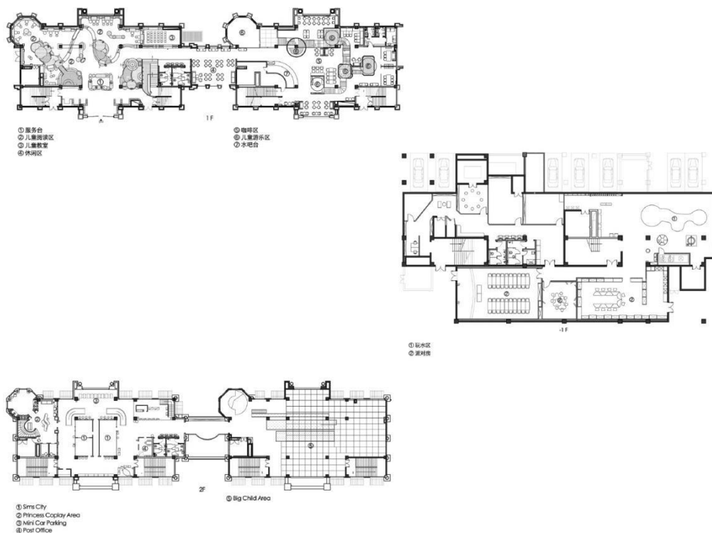
Fig 6.1.4 floor plans
