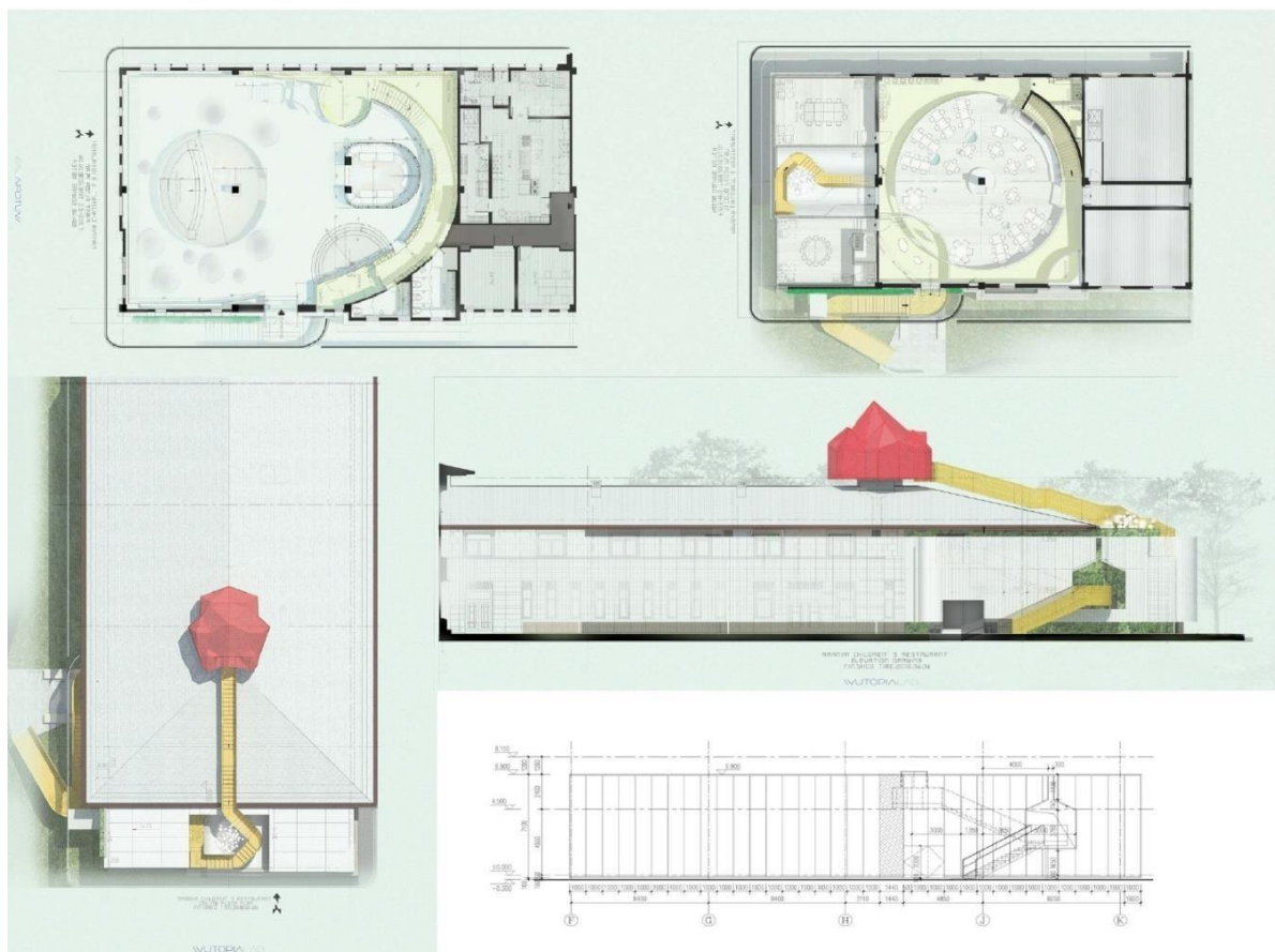
Fig 6.7.2 Planning concept
