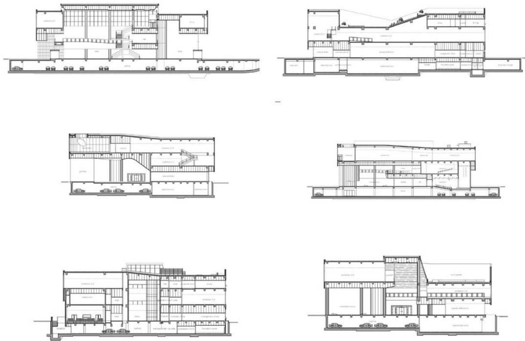
Fig 6.4.3 Plan,elevation,sections
