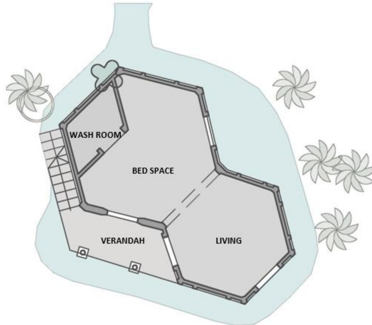
PROTOTYPE PLAN
