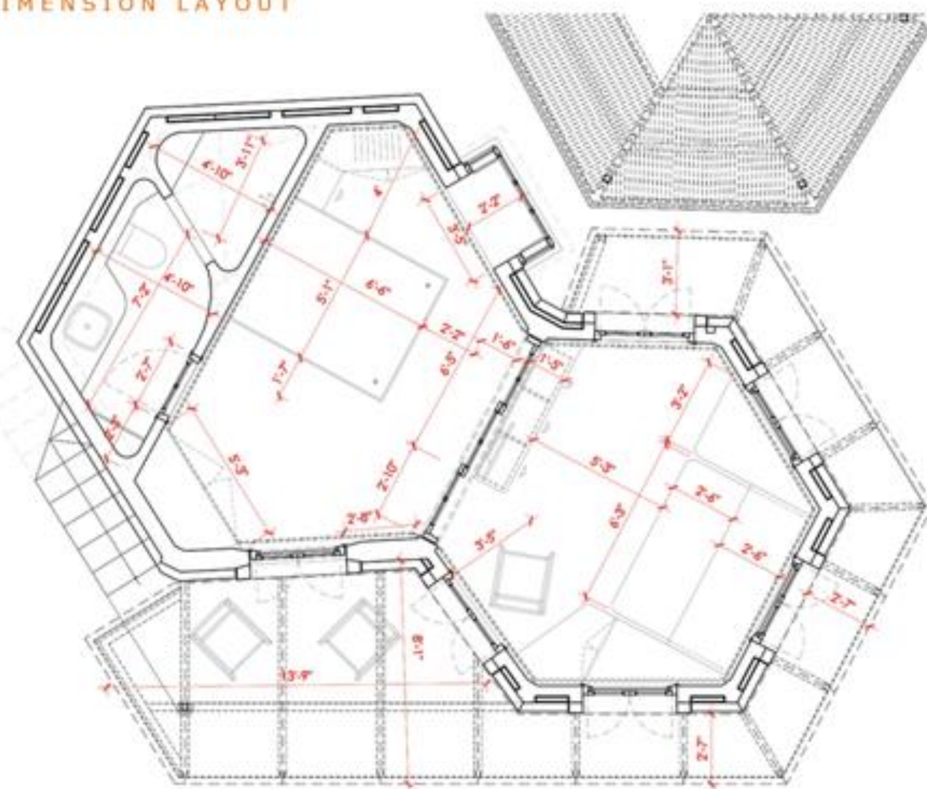
DIMENSION LAYOUT
