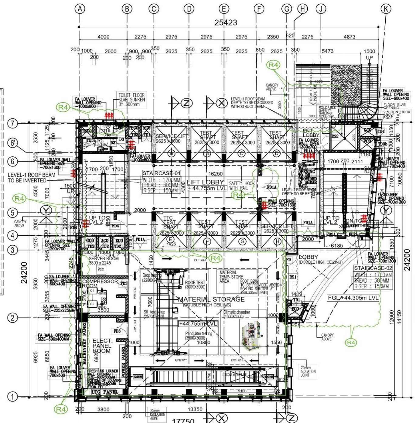
LEVEL : 1 GROUND FLOOR PLAN
