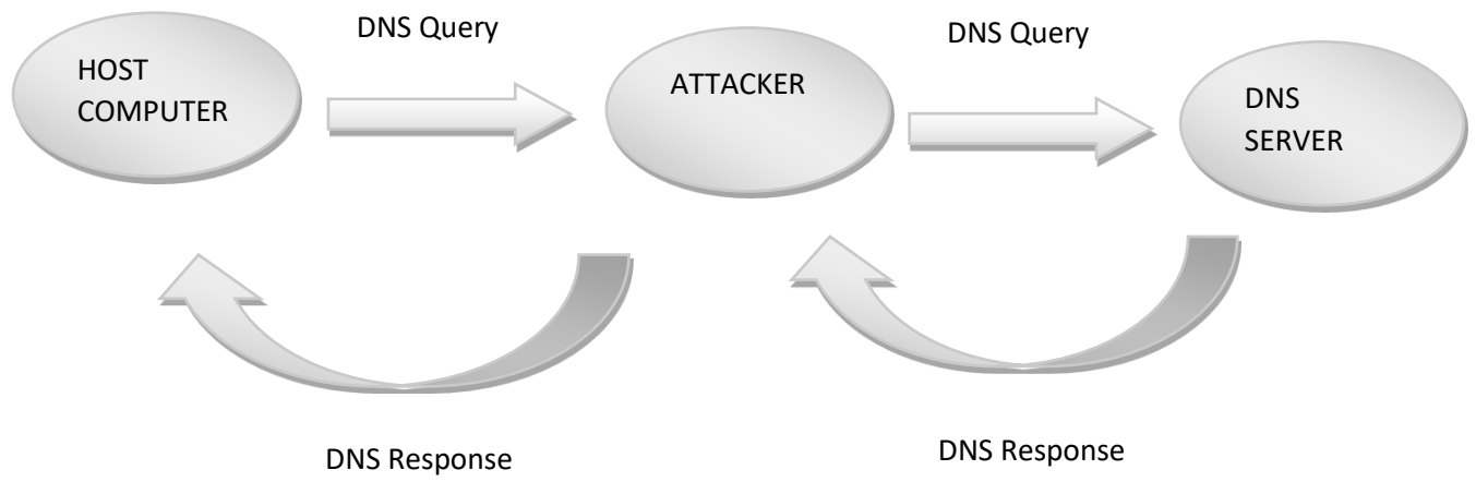
Fig 4.9 DFD-Level 2:
