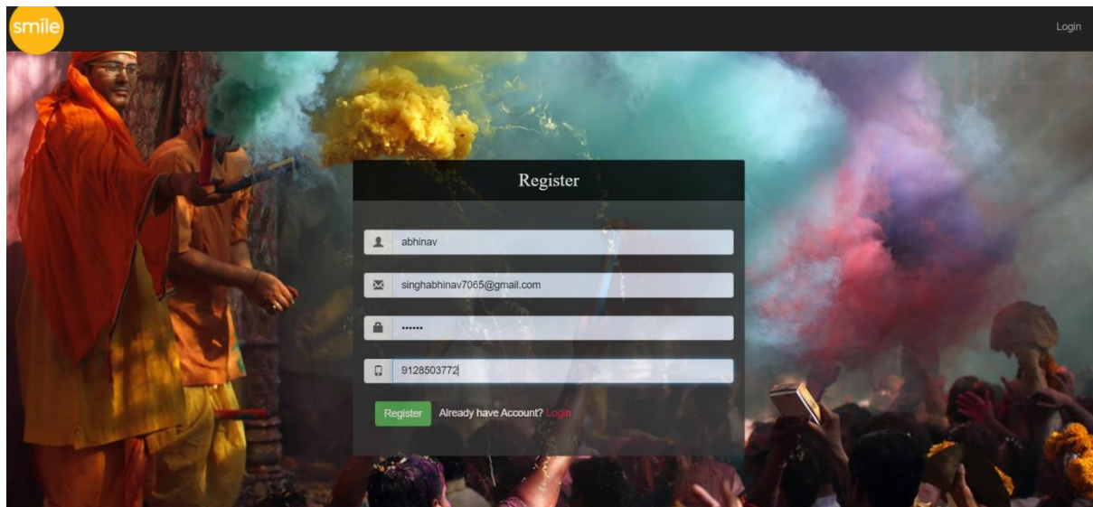
Fig 1.2: Register Page
