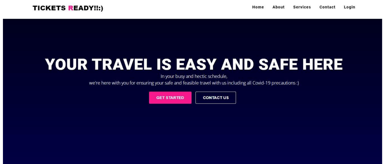
Fig 1.1: Home Page
