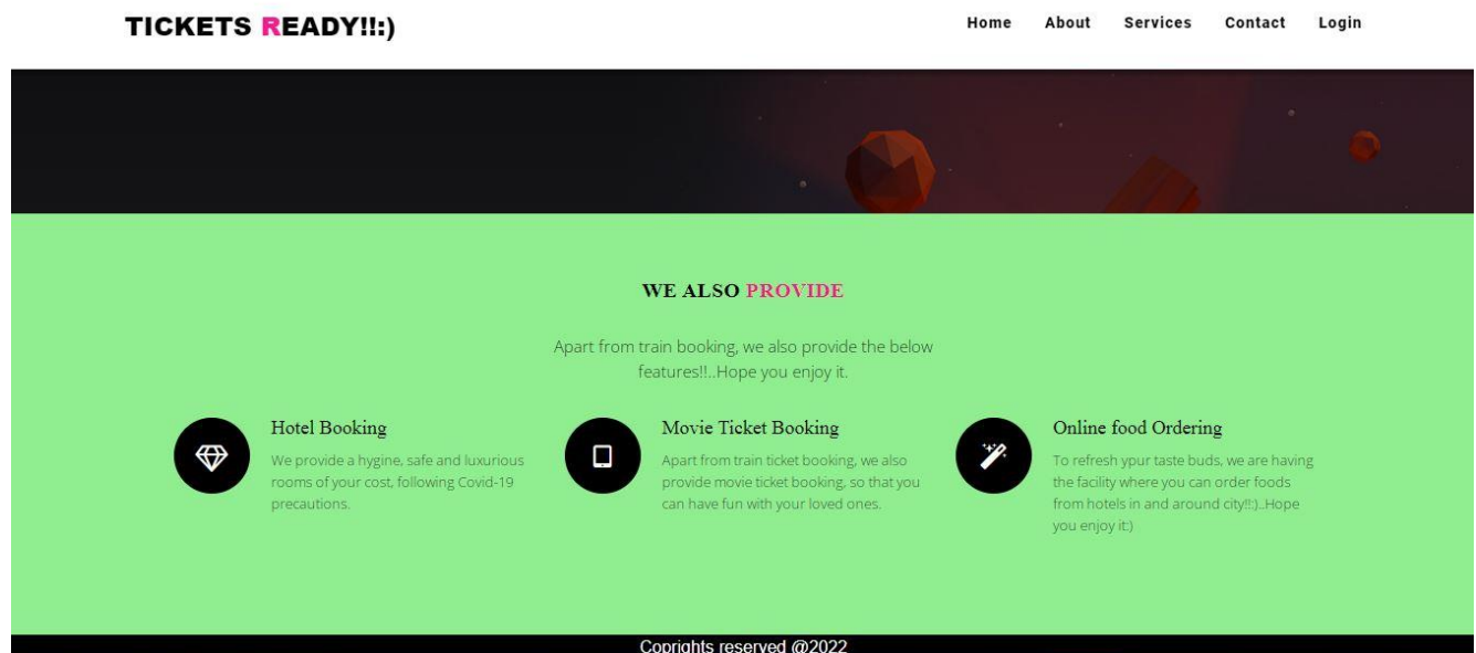
Fig 1.4: Services Page
