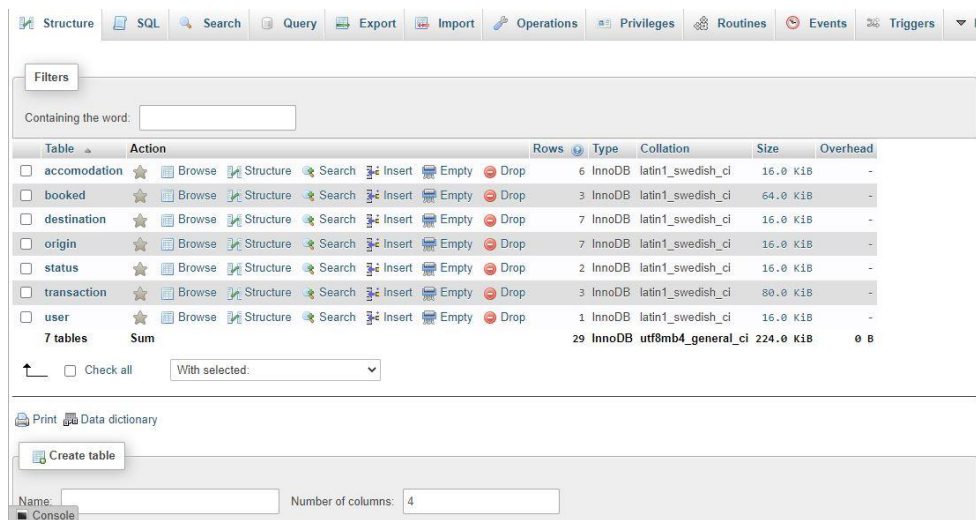
Fig 2: MYSQL Connection
