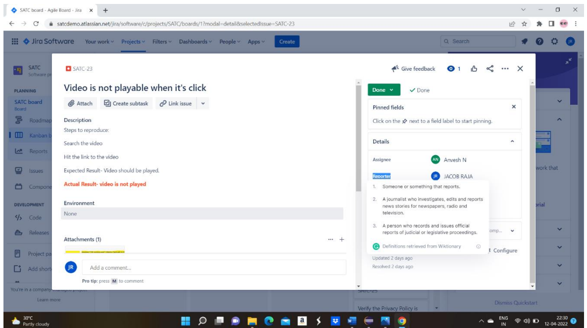
Fig no:1.11.2 Identify the defect and report it to the bug
