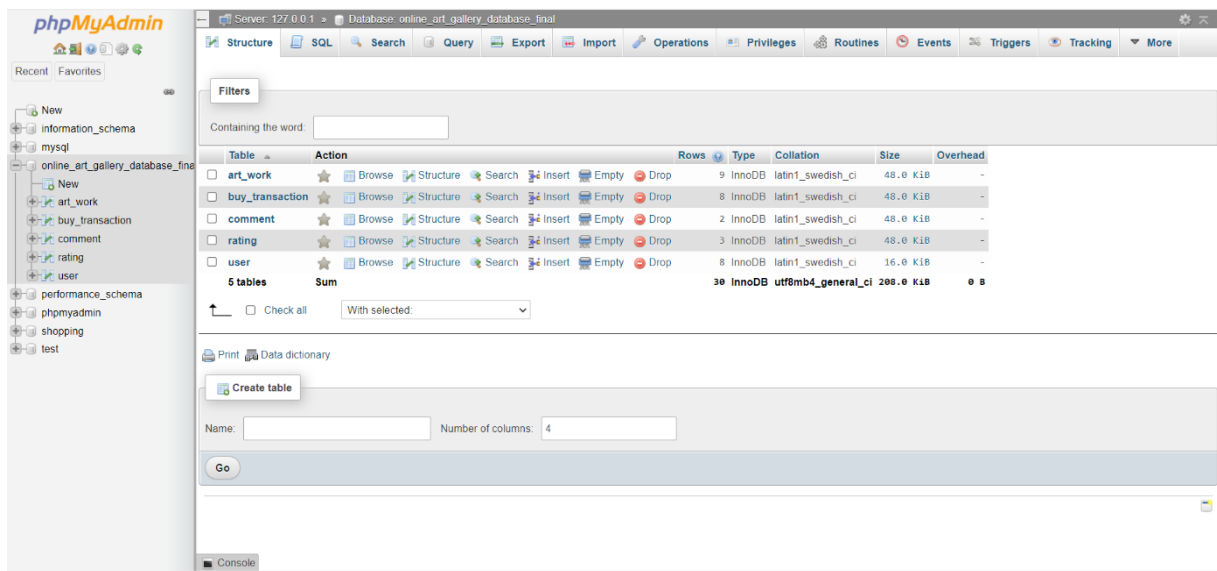
Figure 1.9 MYSQL connection
