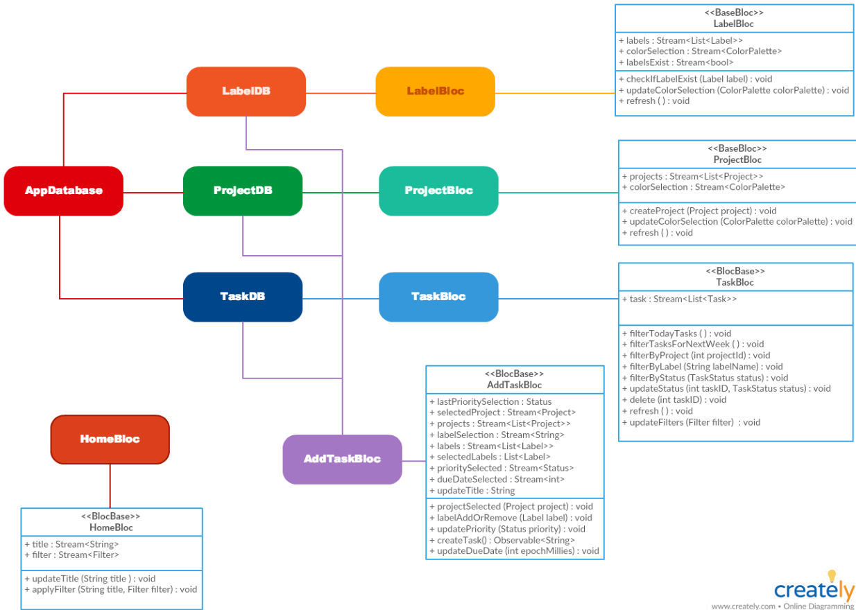
Fig 7: app flowchart
