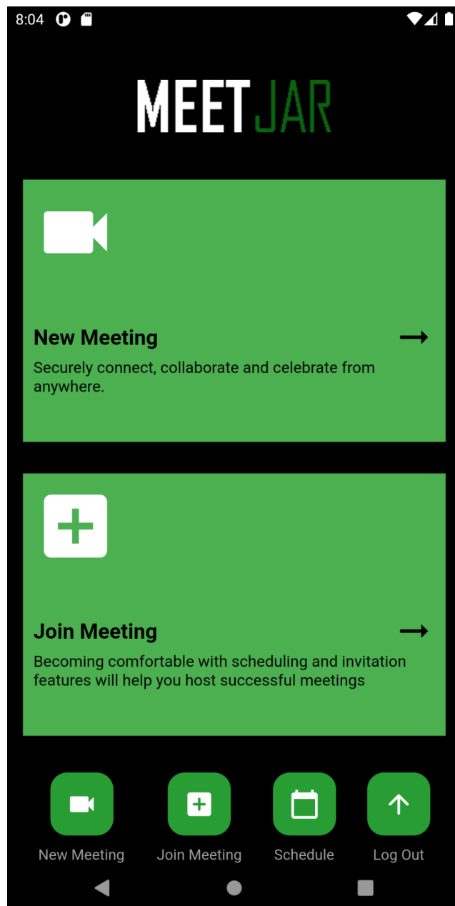
Fig 11: Dashboard
