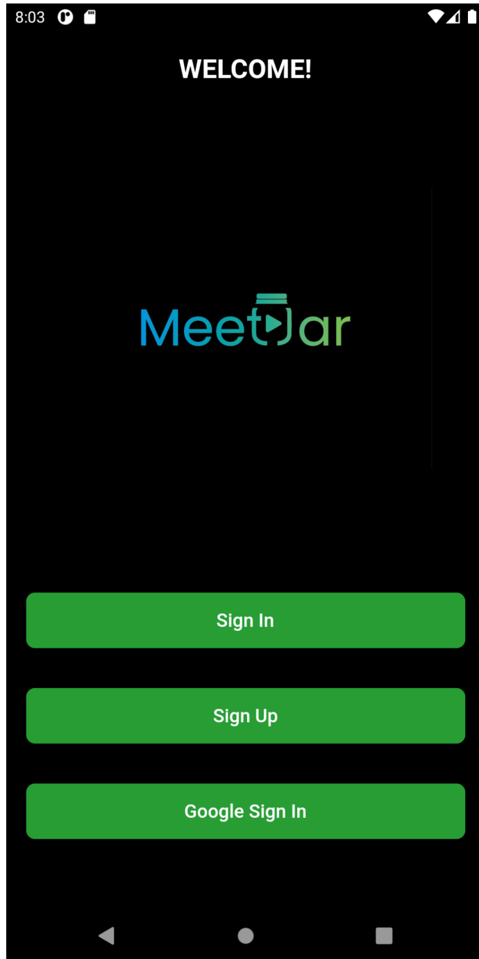
Fig 8: Welcome page
