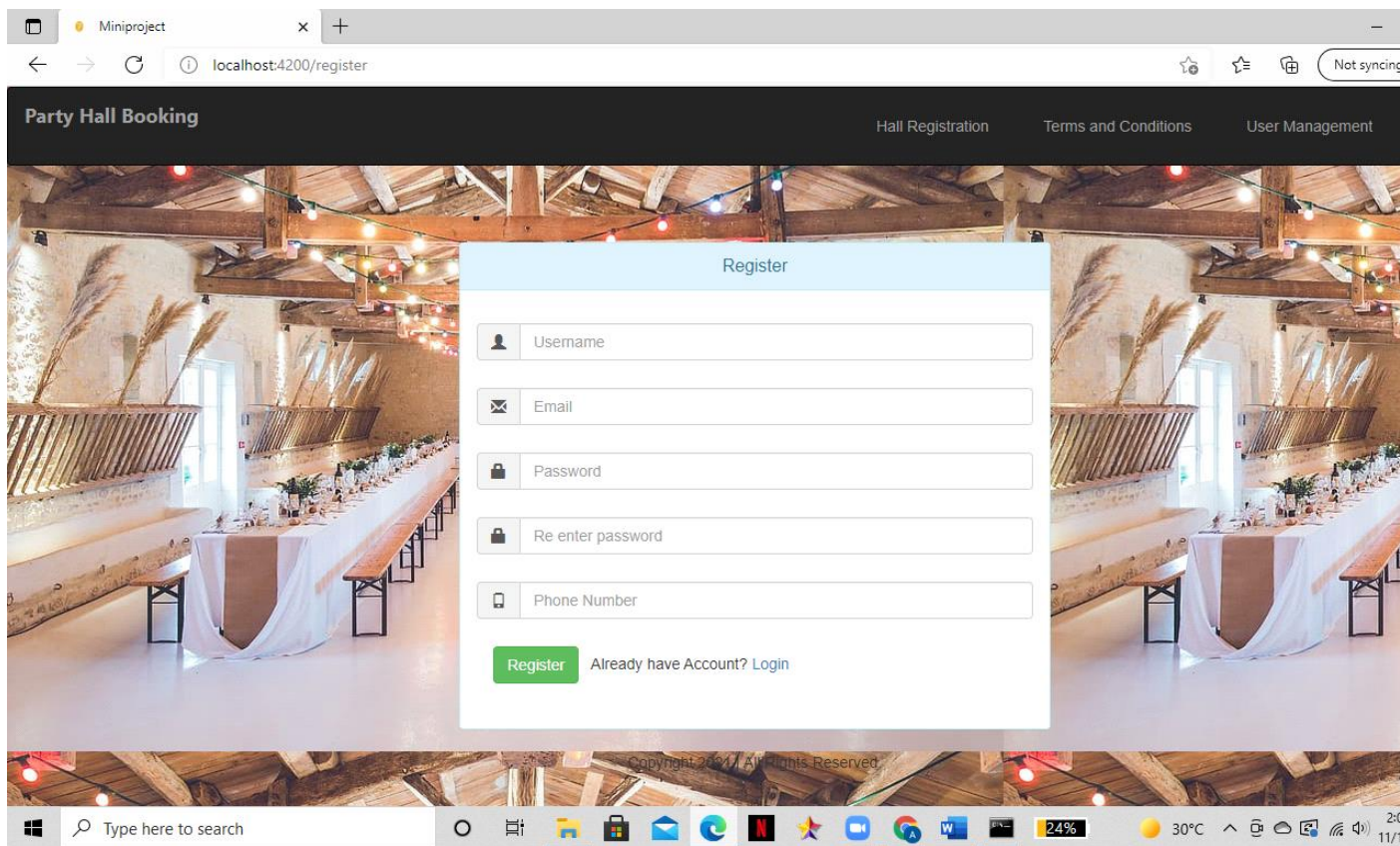
Fig 1.2 : Register Page
