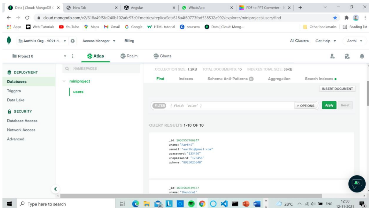
Figure 1.9 MongoDB connection
