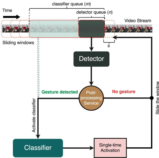
Fig. 2: The general workflow of the proposed two-model hierarchical architecture. Sliding windows with stride s run through incoming video frames where detector queue placed at the very beginning of classifier queue. If the detector recognizes an action/gesture, then the classifier is activated. The detector's output is post-processed for a more robust performance, and the final decision is made using single-time activation block where only one activation occurs per performed gesture.
