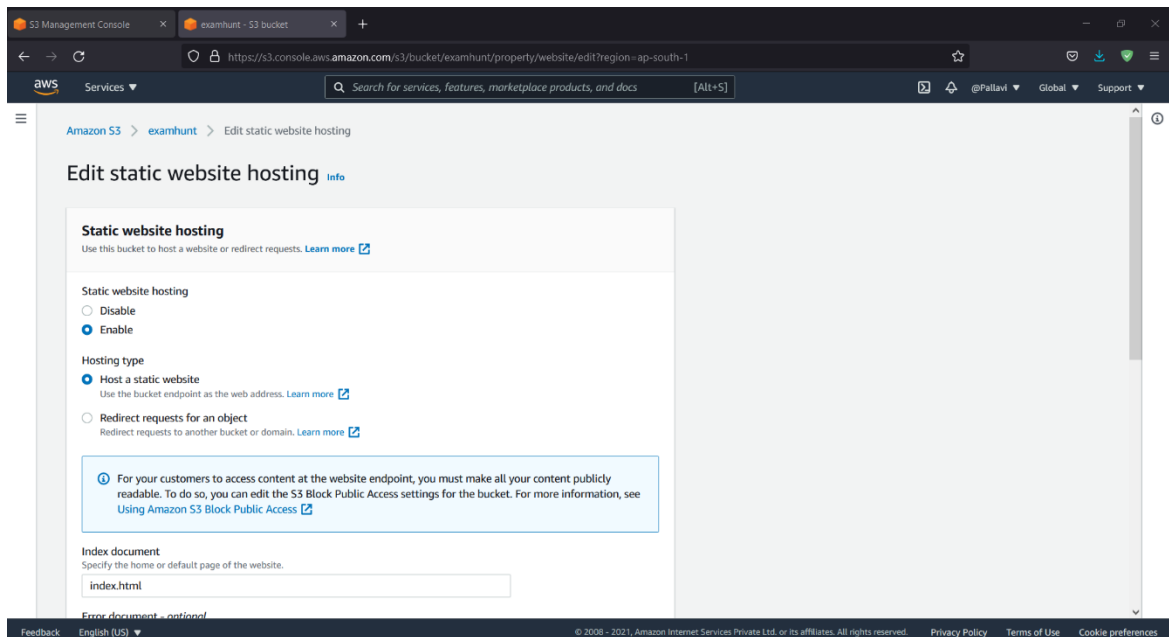
Fig 1.8: Enabling static hosting
