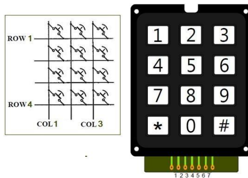
Figure 3. 3: Keypad 4x4
