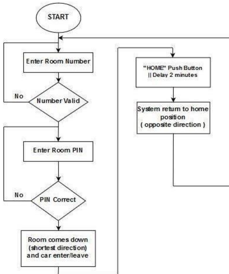
Figure 5. 3: System Flowchart
