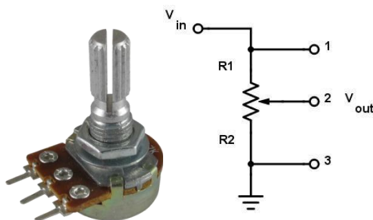
Figure 3. 11: The potentiometer
