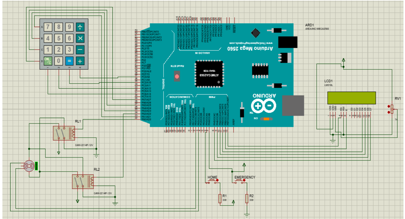
Figure 5. 2: Connection circuit
