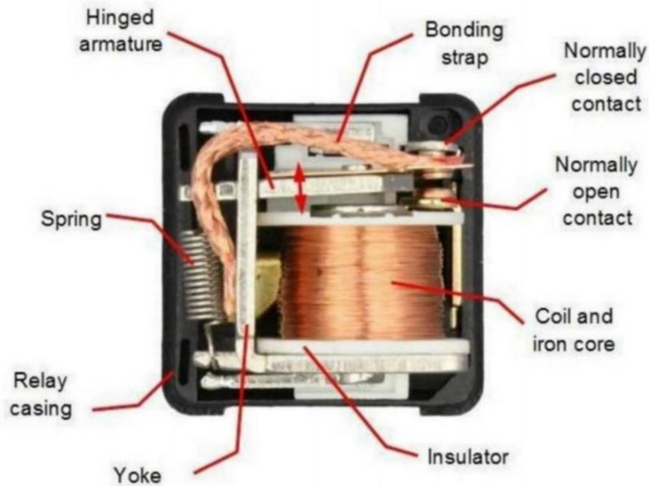
fig.3.1.3. Relay internal structure
