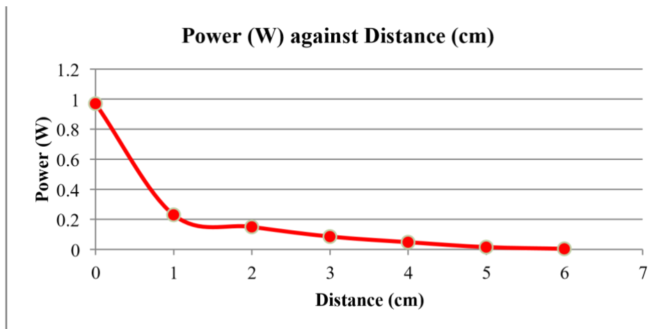
FIGURE 19. Graph of Power (W) against Distance (cm)
