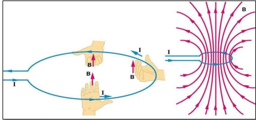
FIGURE 5. Ampere Law [19]
