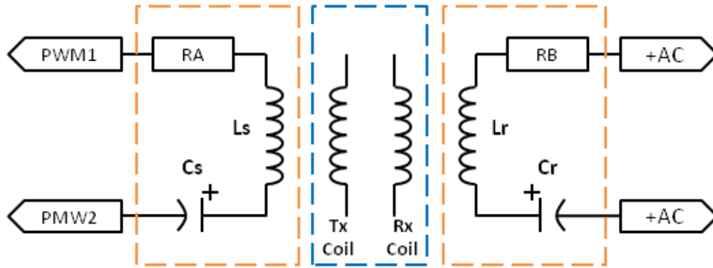
FIGURE 7. Schematic Diagram of the Magnetic Resonant Coupling
