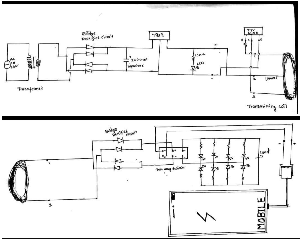
FIG 9. Circuit Diagram of Power Supply Unit
