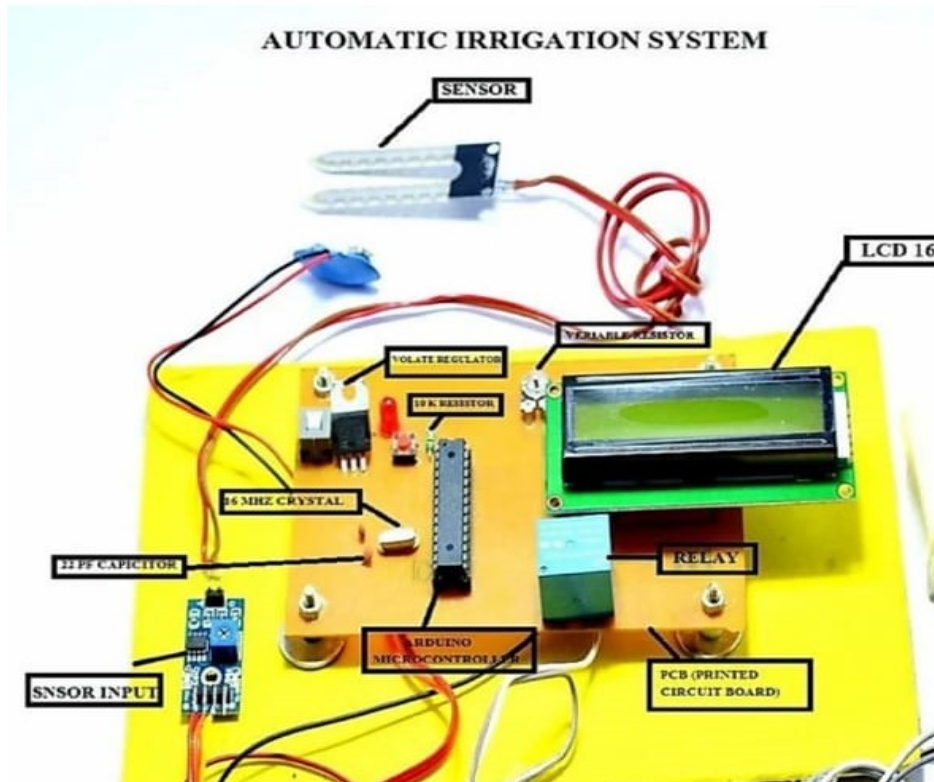
Hardware Model of the System
