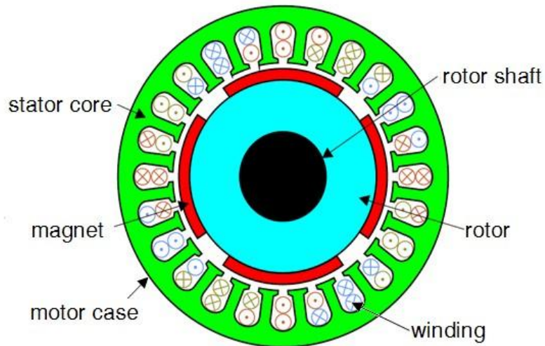
PMSM Structure
