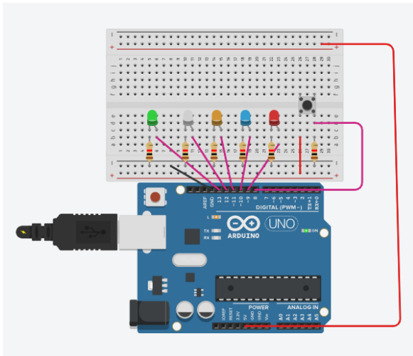
FIG 13.2 PUSH BUTTON
