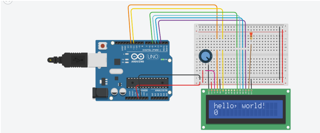
FIG 13.1 HELLO WORLD
