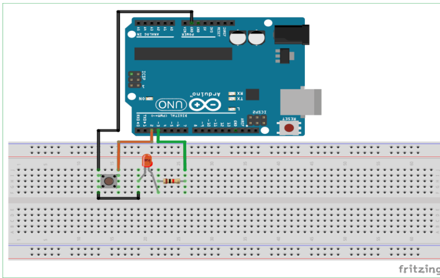
FIG12.2 CONNECTION DIAGRAM OF BUTTON LED
