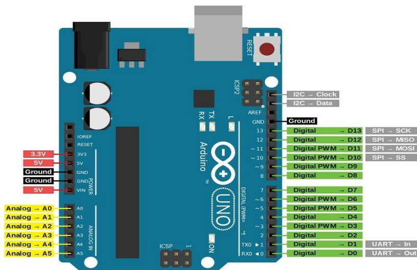
FIG 11.4 PIN DIAGRAM
