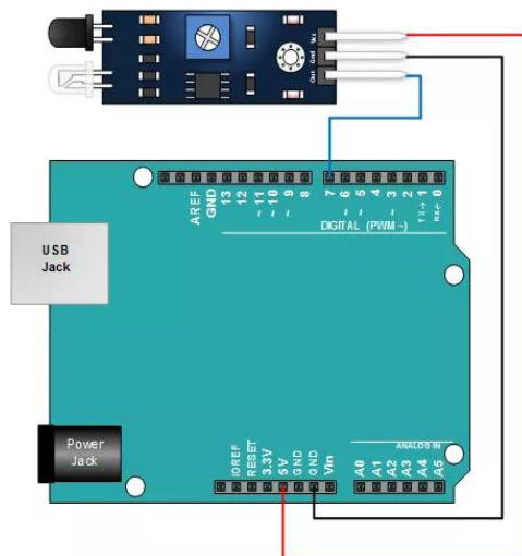
FIG12.3 CONNECTION DIAGRAM OF IR SENSORS
