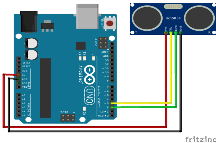
FIG12.4 CONNECTION DIAGRAM OF ULTRASONIC SENSORS
