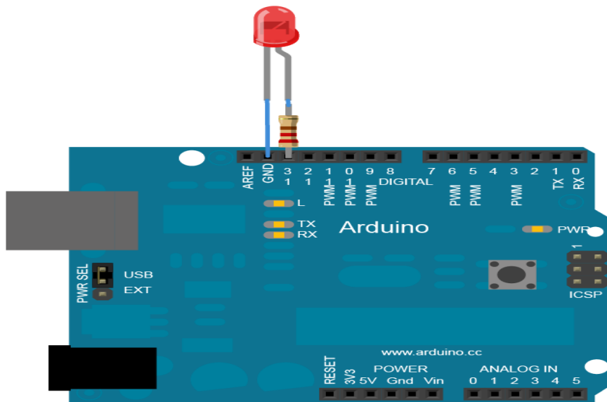
FIG12.1 CONNECTION DIAGRAM OF LED BLINKING
