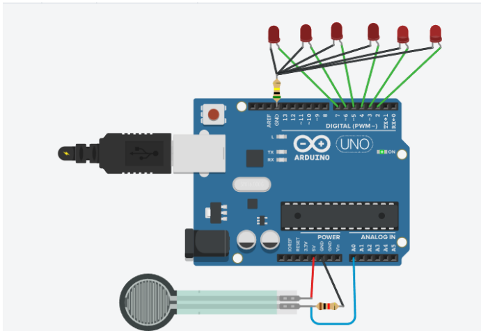
FIG 13.3 LEDs
