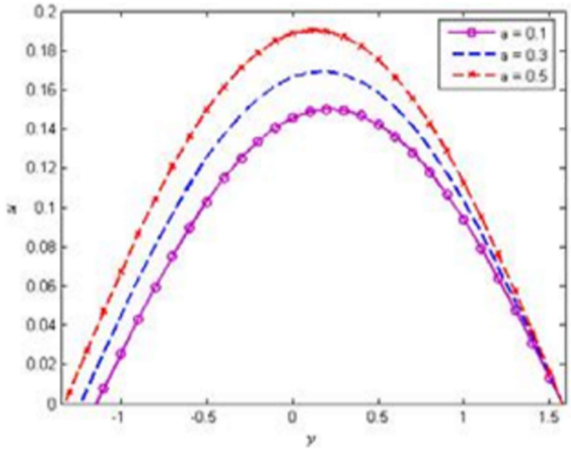
Figure 5. 2: Variation of m on u for a = 0.3 , b = 0.5 , \phi = \pi/4 , x = 0.5 , m = 0.5 , t = 0.2 , S = 0.5 .
