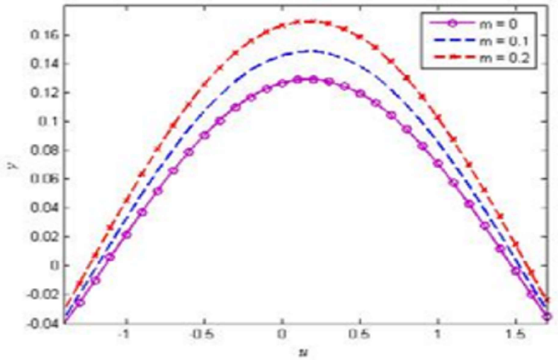
Figure 5.3: Variation of m on u for a = 0.3 , b = 0.5 , \phi = \pi / 4 , x = 0.5 , t = 0.2 , S = 0.5 .
