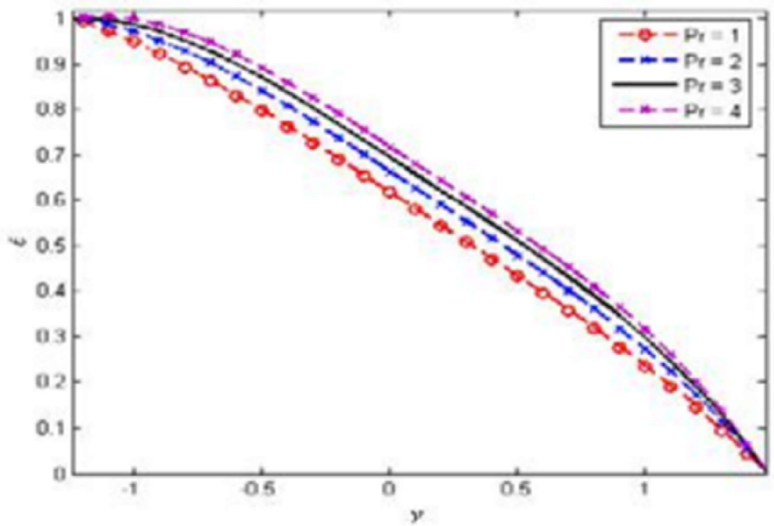
Figure 5.7: Variation of Pr on \Theta for a = 0 , b = 0.4 , \phi = \pi , x = 0.5 , Rn = 0.3 , m = 0.2 , t = 0.2 , E = 0.75 , S = 1.5
