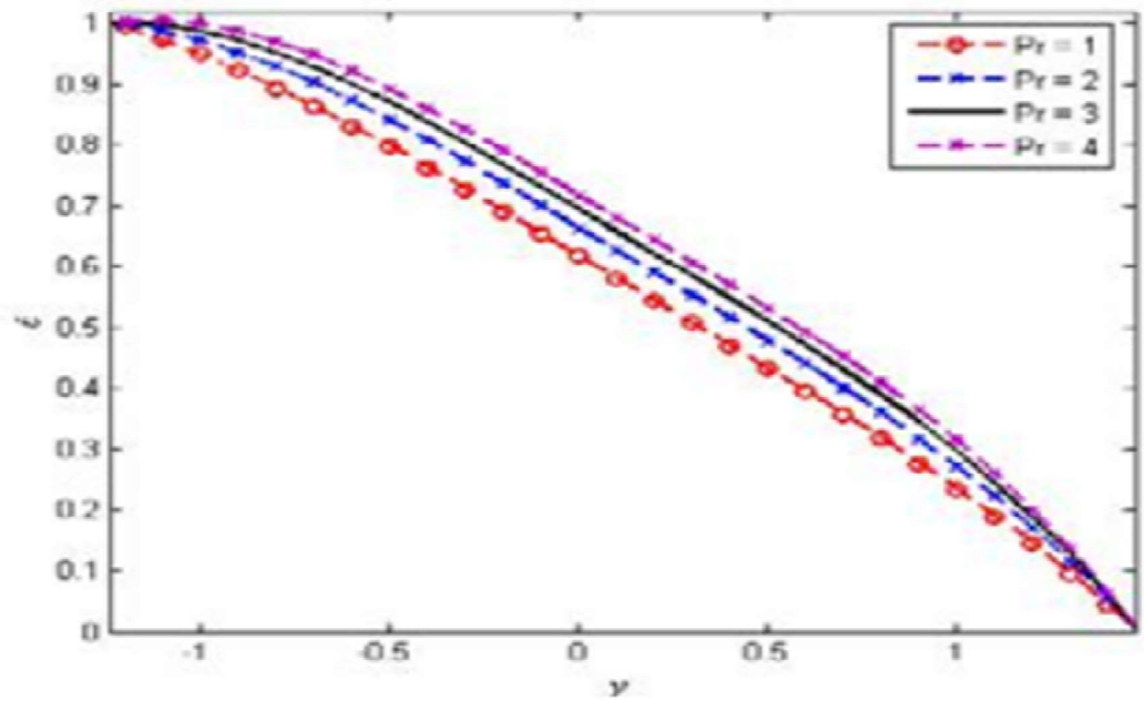
Figure 5.6: Variation of E on \Theta for a = 0.3 , b = 0.4 , \phi = \pi , x = 0.5 , m = 0.2 , t = 0.2 , Rn = 0.3 , Pr = 6.2 , S = 1.5 .
