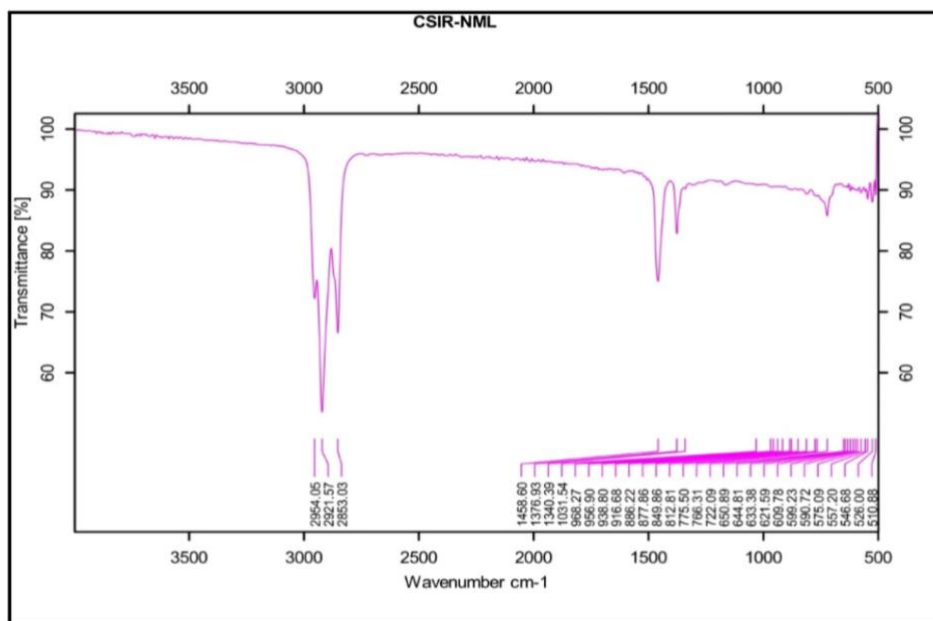
FTIR Spectrum of the Diesel Oil.
