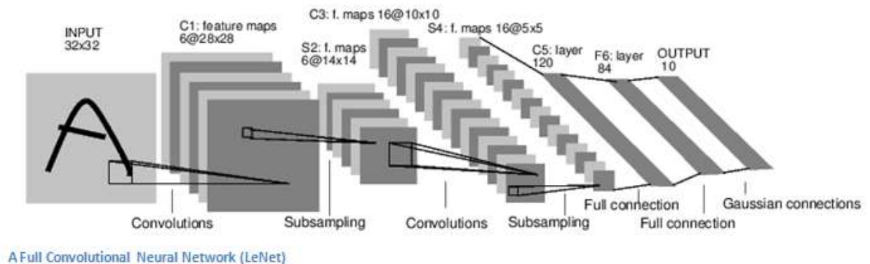
Fig.4.4.5.:CNN diagram
