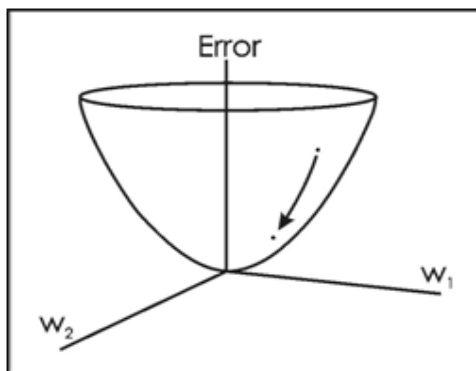
Fig.4.4.6.:Error Image
