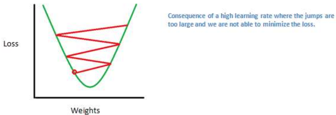
Fig.4.4.7.: Graph Image
