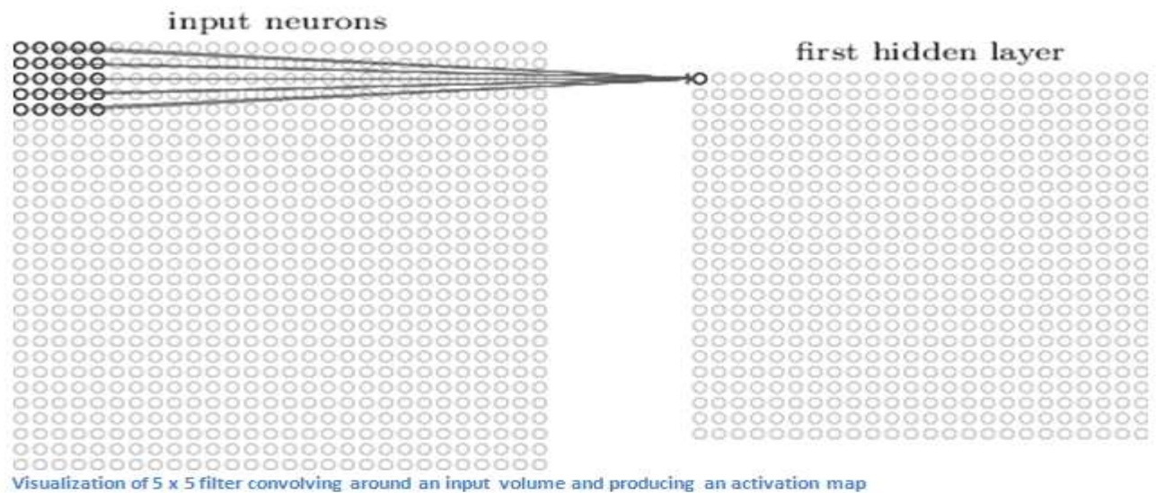
Fig.4.4.2.:Input volume and producing an activation map
