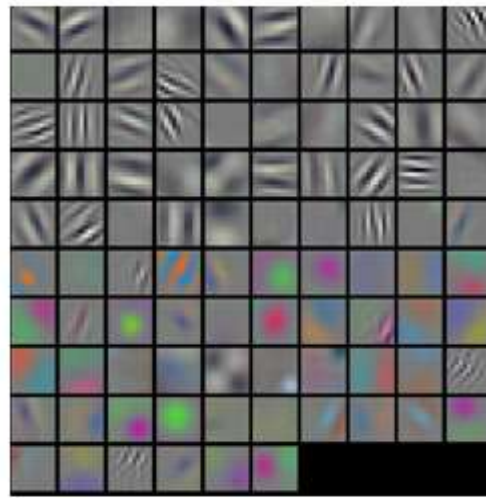
Visualizations of filters
