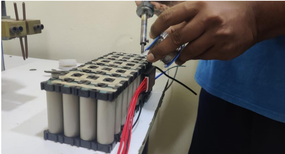
Fig.4.6 connecting cells
