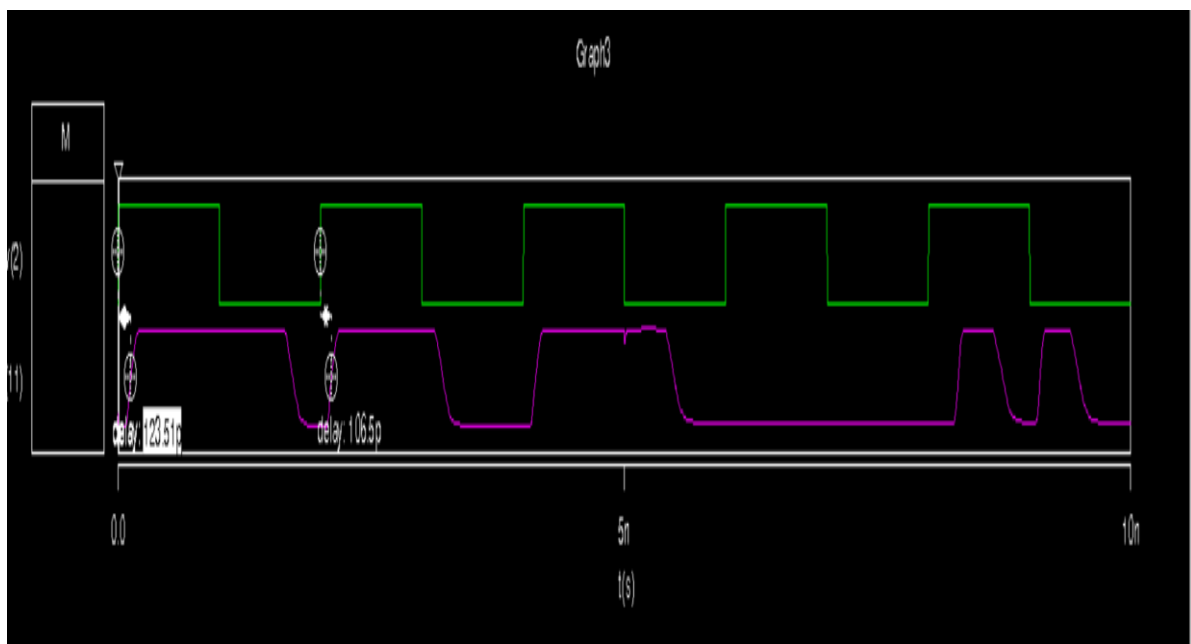
Fig:5.6: Delay analysis of Half adder
