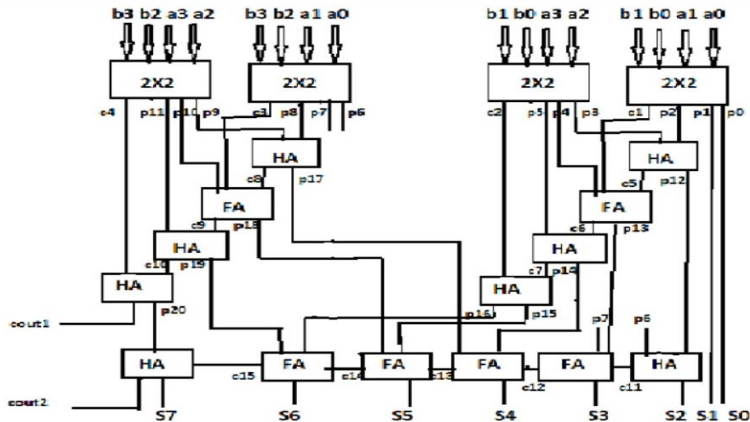
Fig.4.2.3 Proposed 4*4 Multiplier
