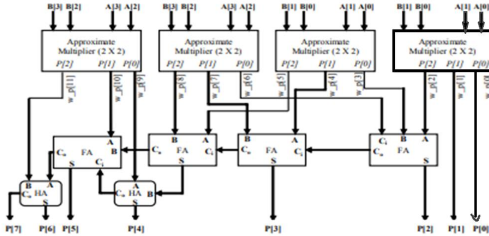
Fig: Logic diagram of existing 4*4 multiplier
