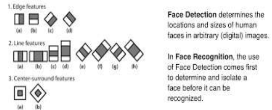
Fig.3 Haar features
