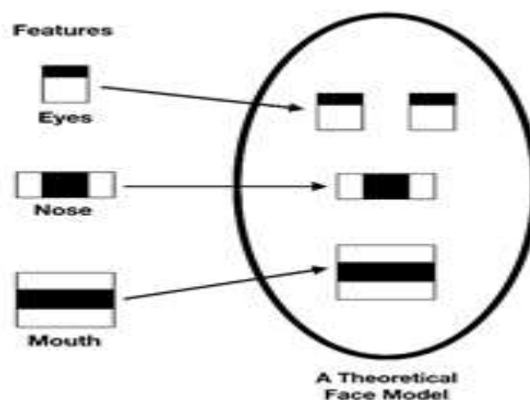
FIGURE 3.3: FEATURE EXTRACTION
