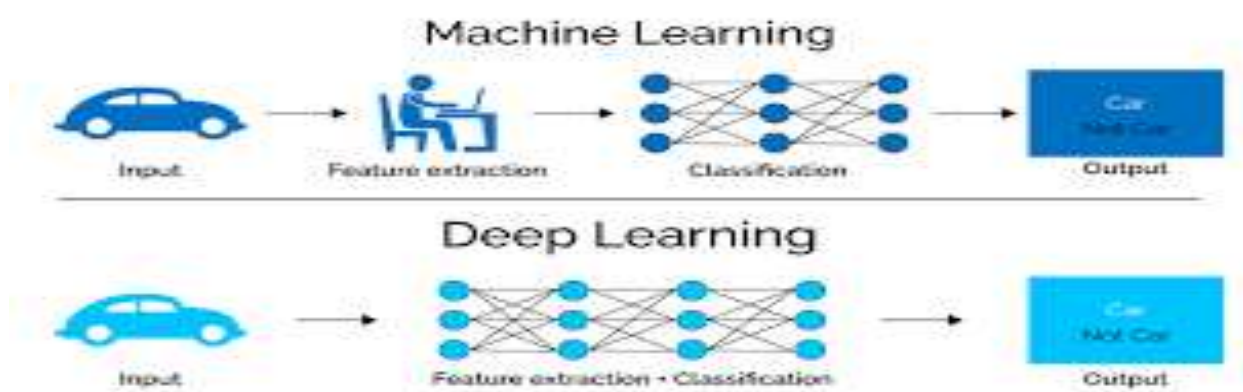
FIGURE 2.1: DEEP LEARNING
