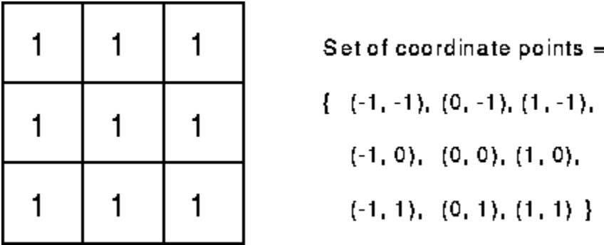
Figure 1 Convolution kernel for a mean filter with 3×3 neighborhood.
