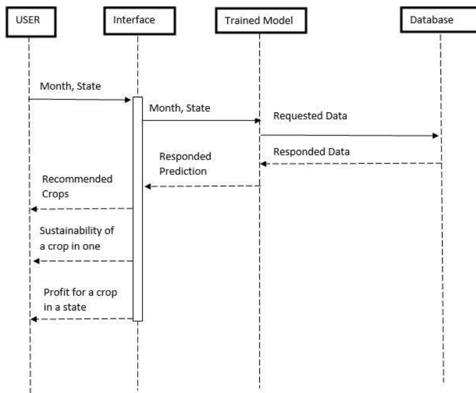
Figure 6.3 Sequence Diagram
