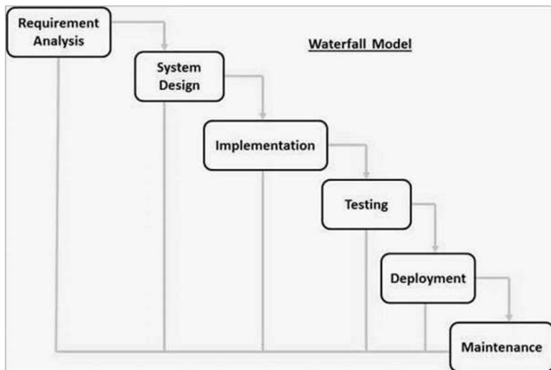
Figure 6.1 Waterfall Model
