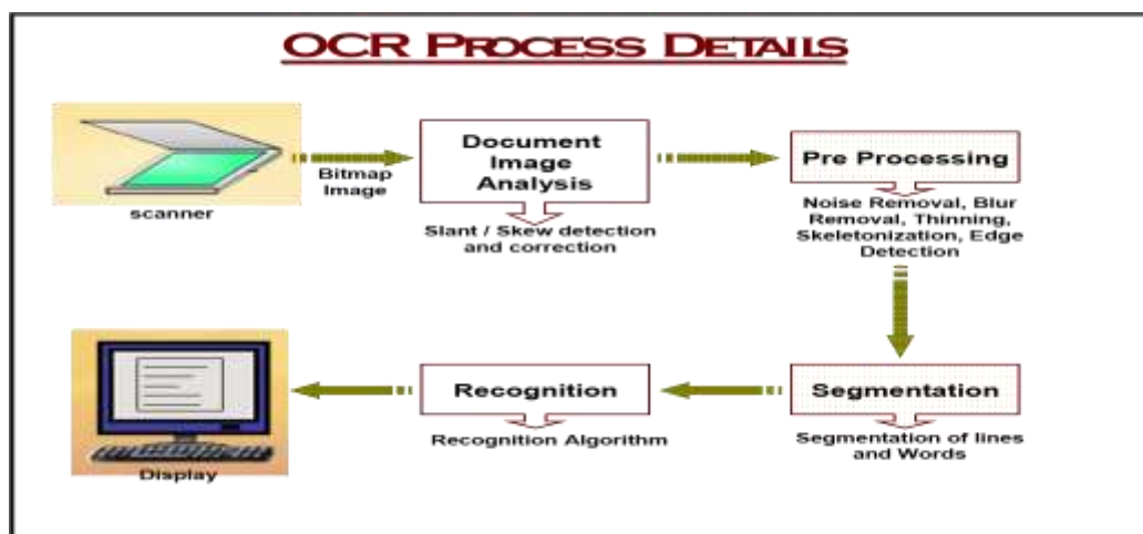
Figure 1.3: OCR Processes
