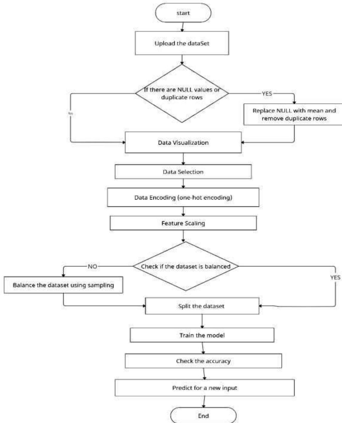
Fig 23: Flow Diagram for Money Laundering Detection
