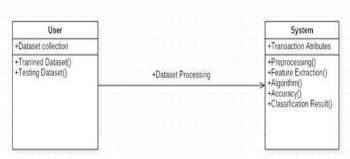
Fig 25: Class Diagram for Money Laundering detection
