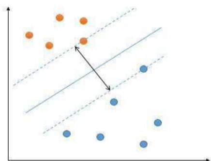
Fig 13: Sample of Support Vector Machine
