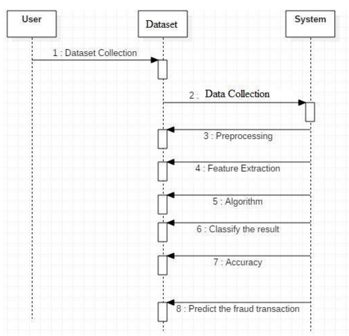
Fig 27: Sequence Diagram for Money Laundering detection
