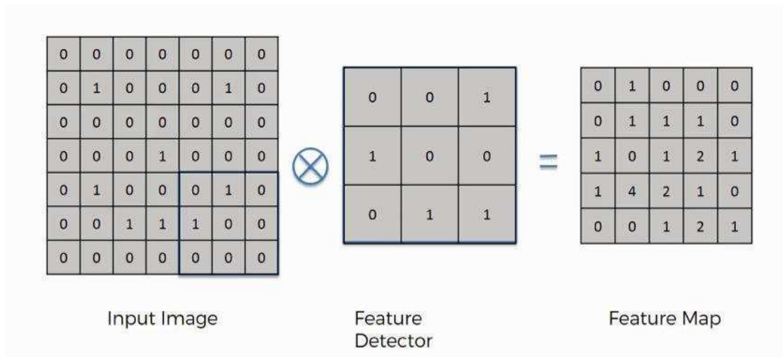
Fig 19: Convolution in CNN Model
