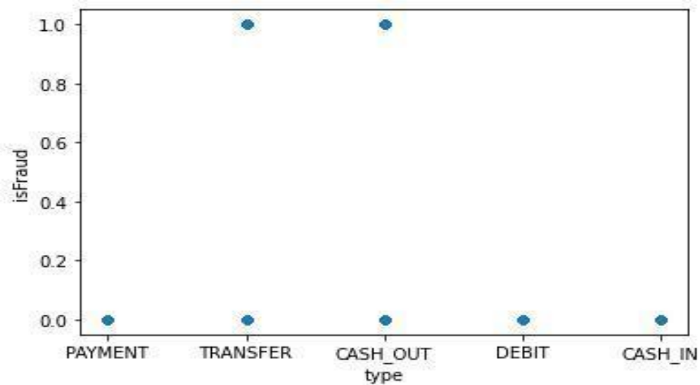
Fig 32: Scatter Plot
