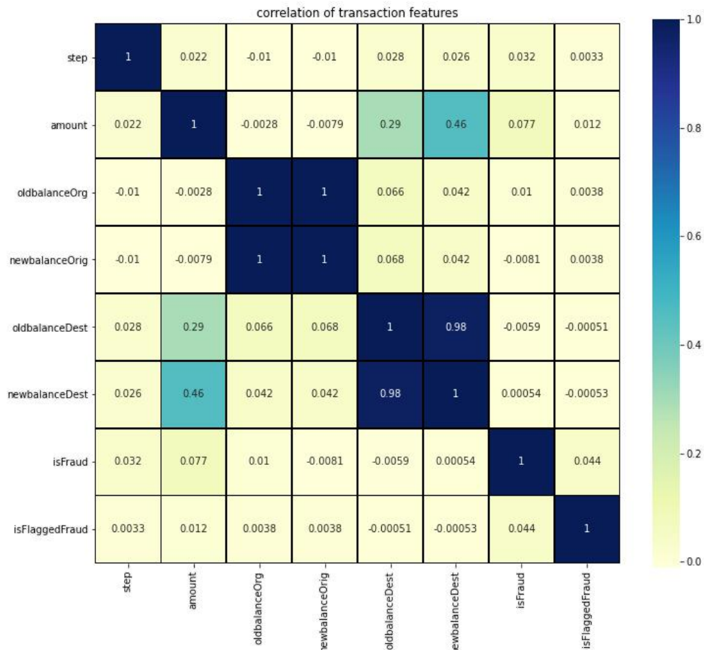
Fig 31: Heapmap
