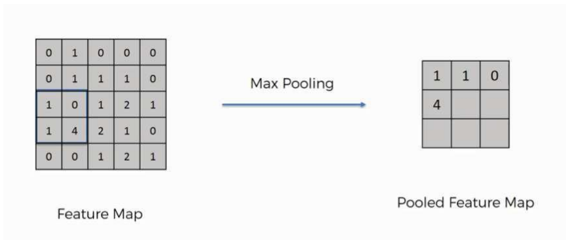
Fig 20: Max Pooling in CNN Model
