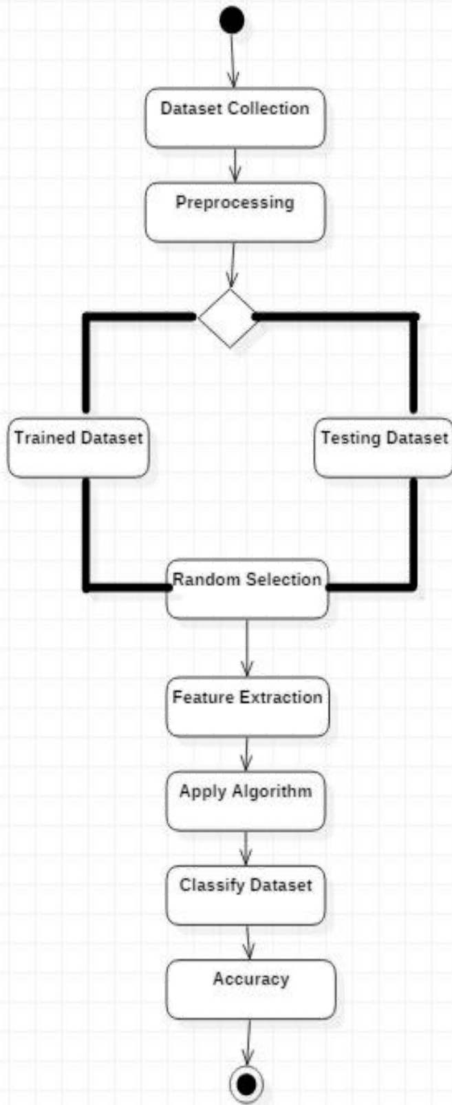
Fig 26: Activity Diagram for Money Laundering Detection
