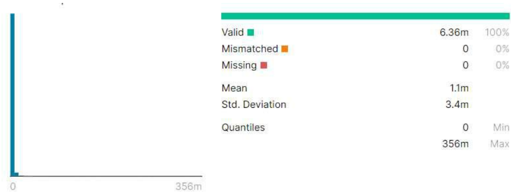
Fig 8: oldbalanceDest attribute statistics
