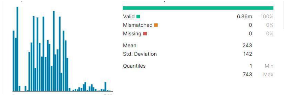
Fig 1: Step attribute statistics
