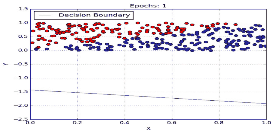
Fig 4.2 Decision Boundary
