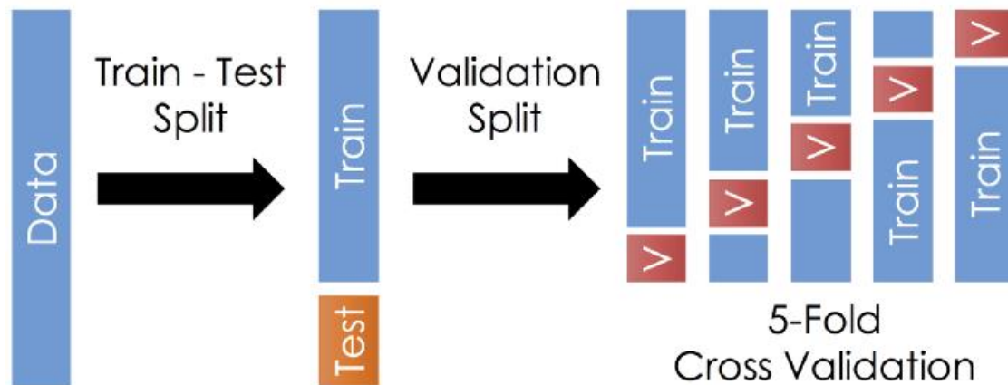
Fig 4.7 Validation Set
