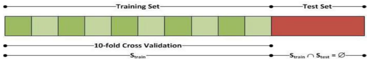
Fig 4.6 Training Set
