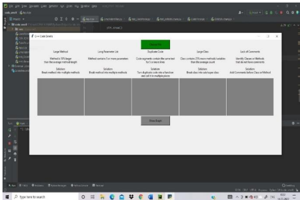
Fig 1 Input Window
