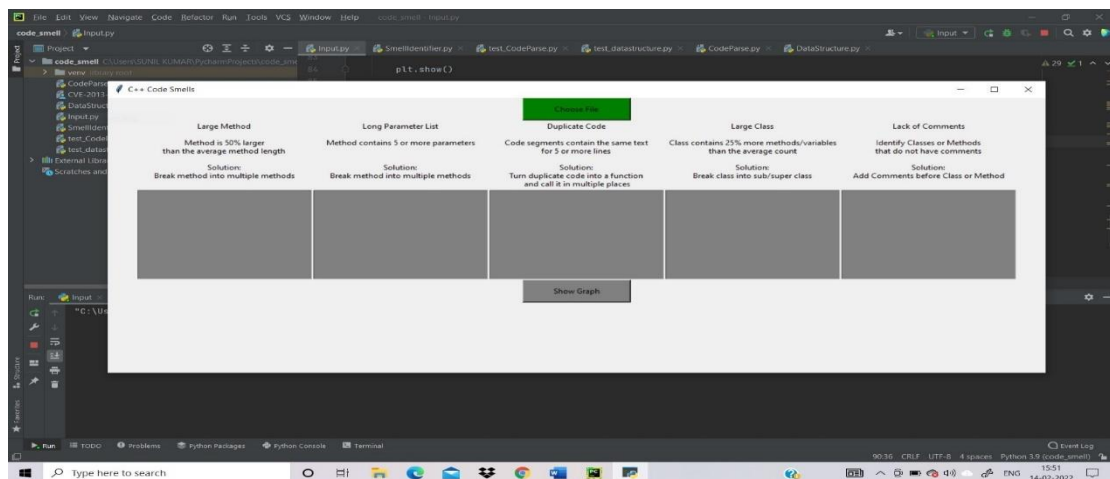
Fig 1 Input Window
