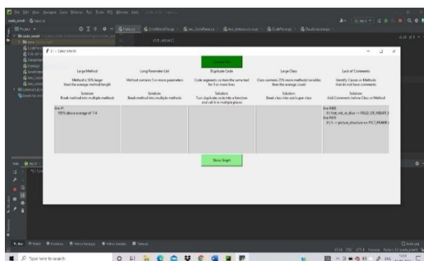
Fig 3 Sample Code Window
