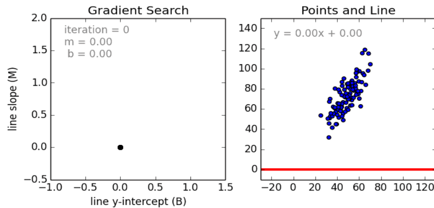
Fig 4.3 Gradient Search and Points and Line
