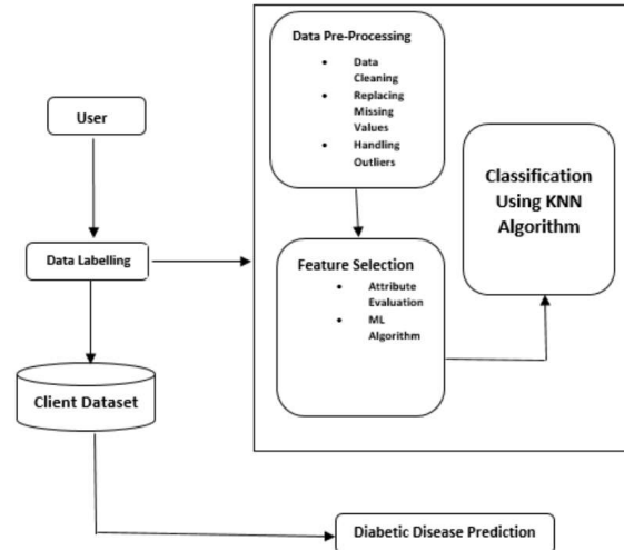
Fig.4.1. Architecture Diagram
