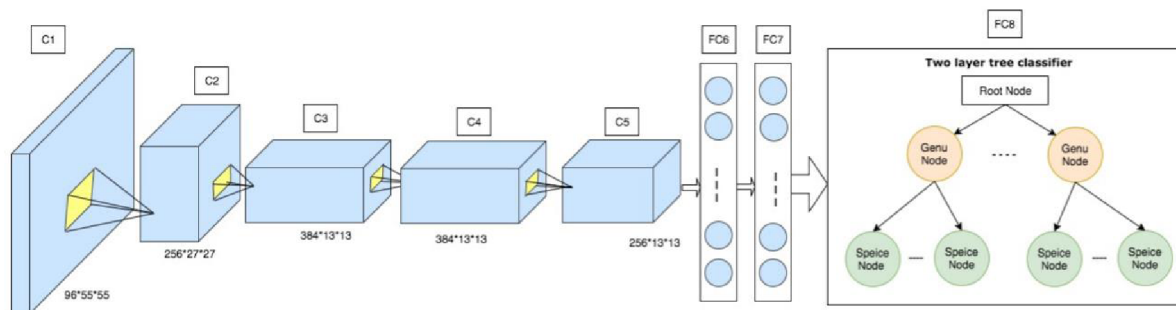
Fig.4.4 ARCHITECTURE DIAGRAM
