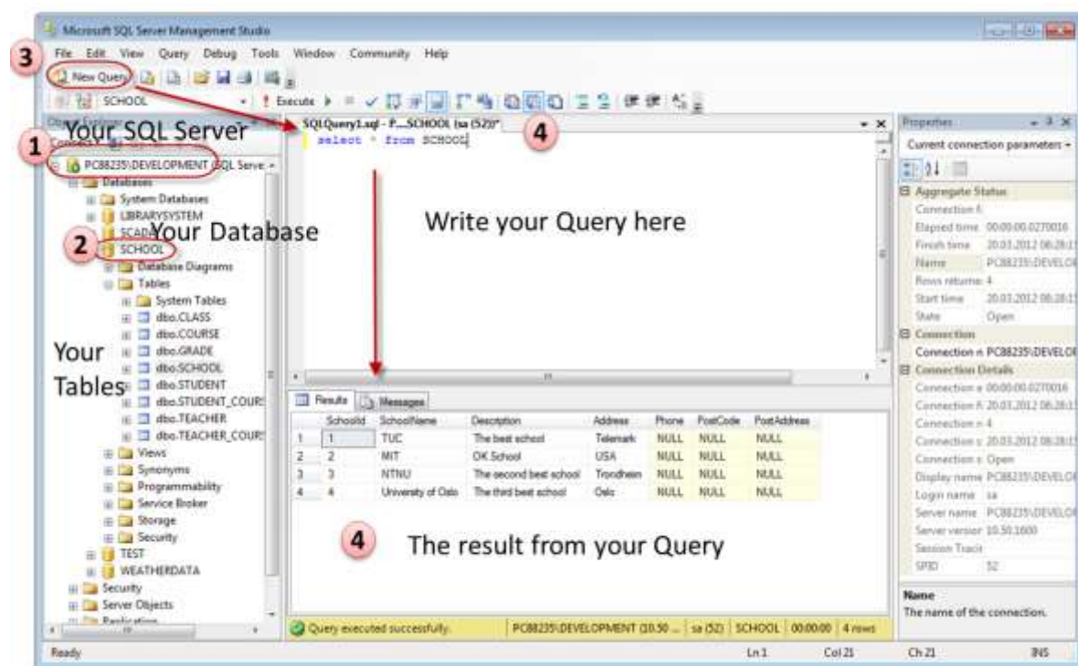
Fig.9. Query Editor
