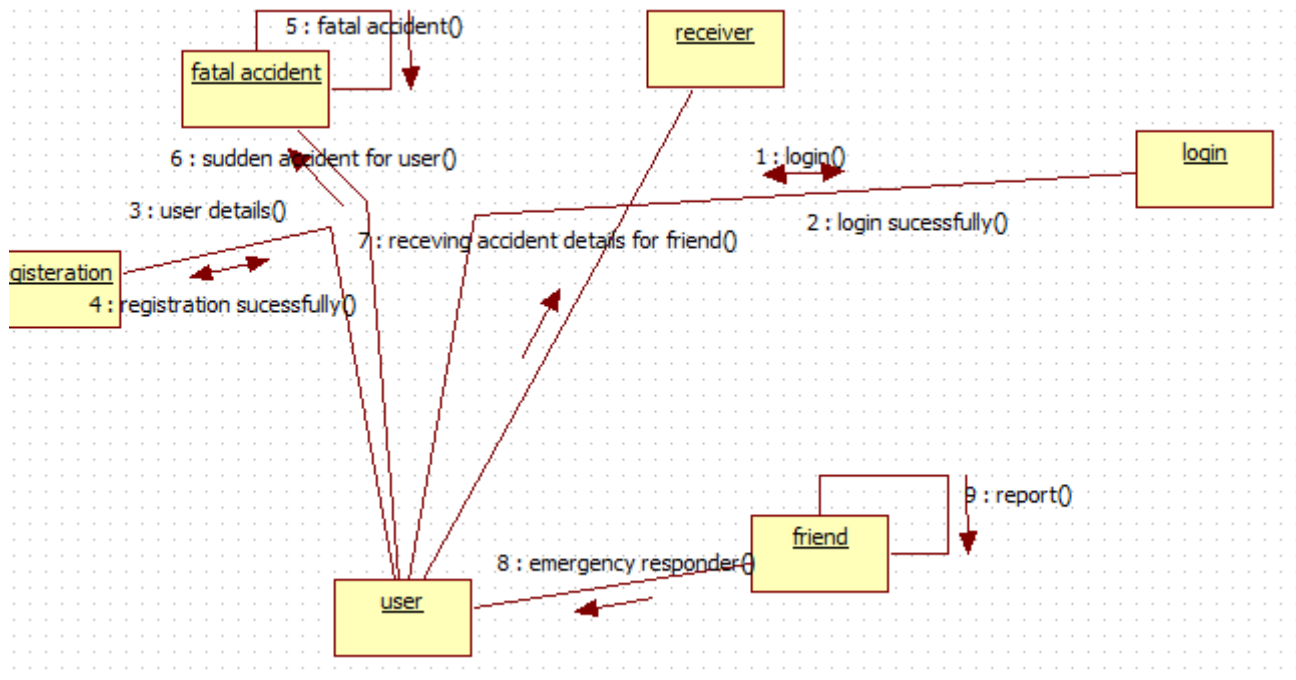
Fig.5. Collaboration diagram
