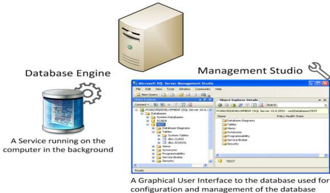
Fig.8. Management Studio
