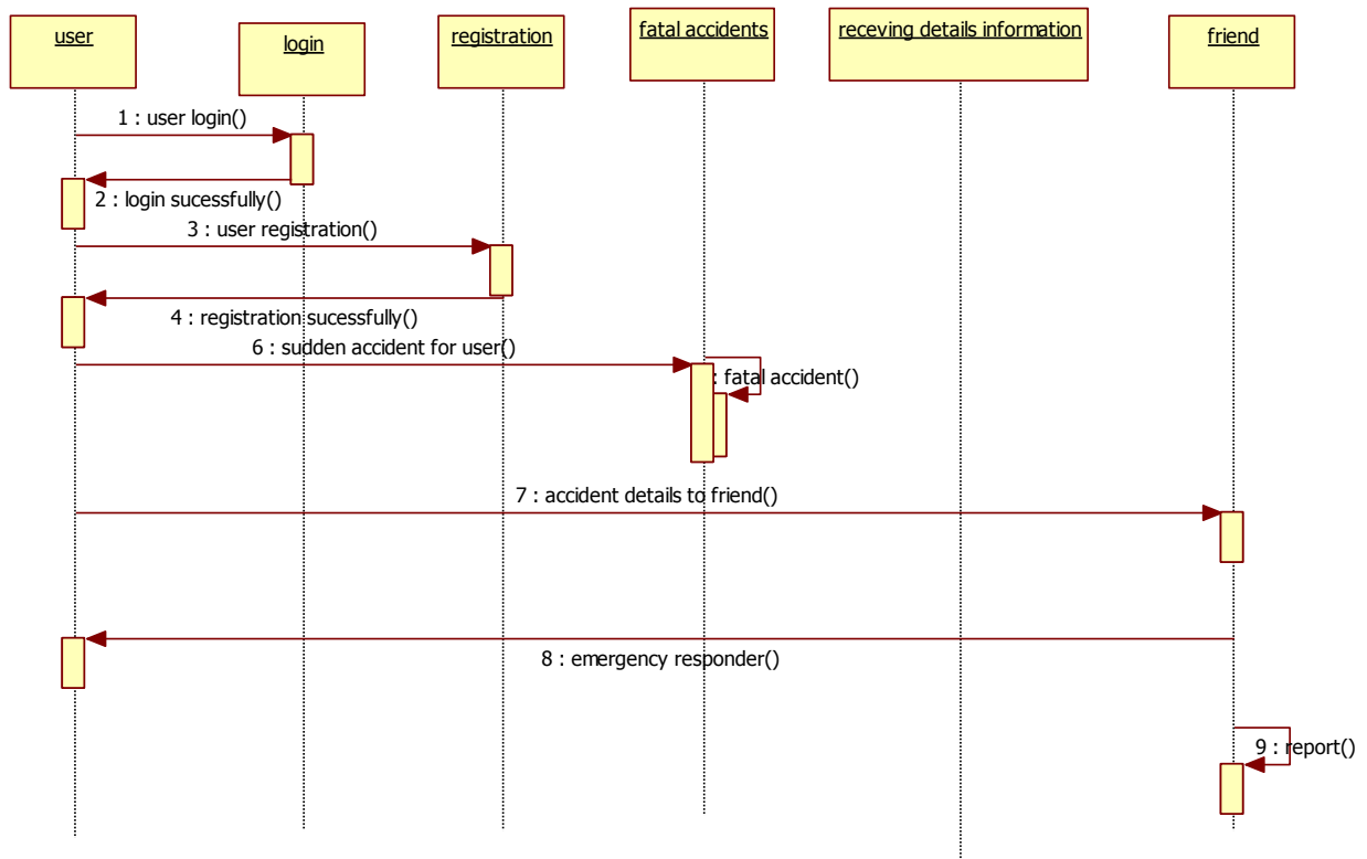
Fig.4. Sequence diagram
