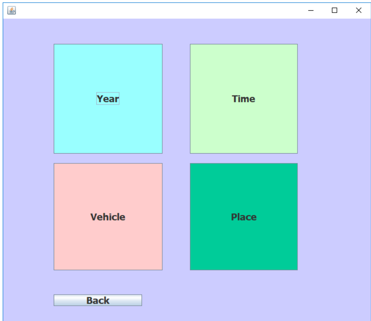
Fig.10. STATITICAL INFORMATION
