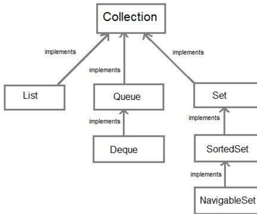
Fig.7. Collection Framework
