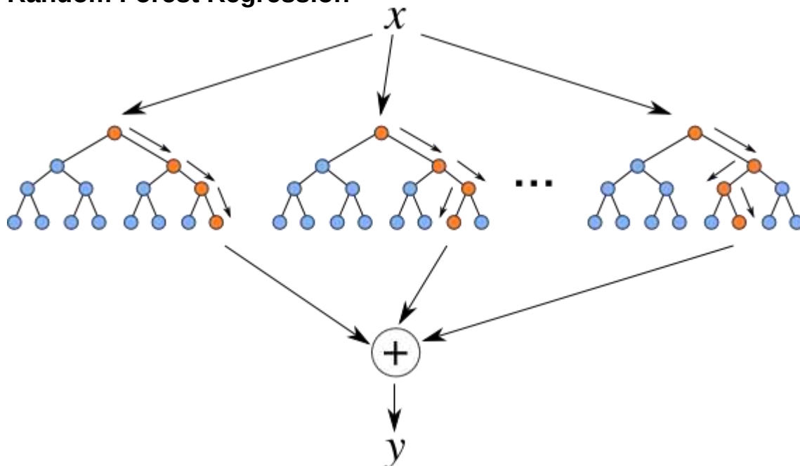
Figure 8 – Procedure of random forest
