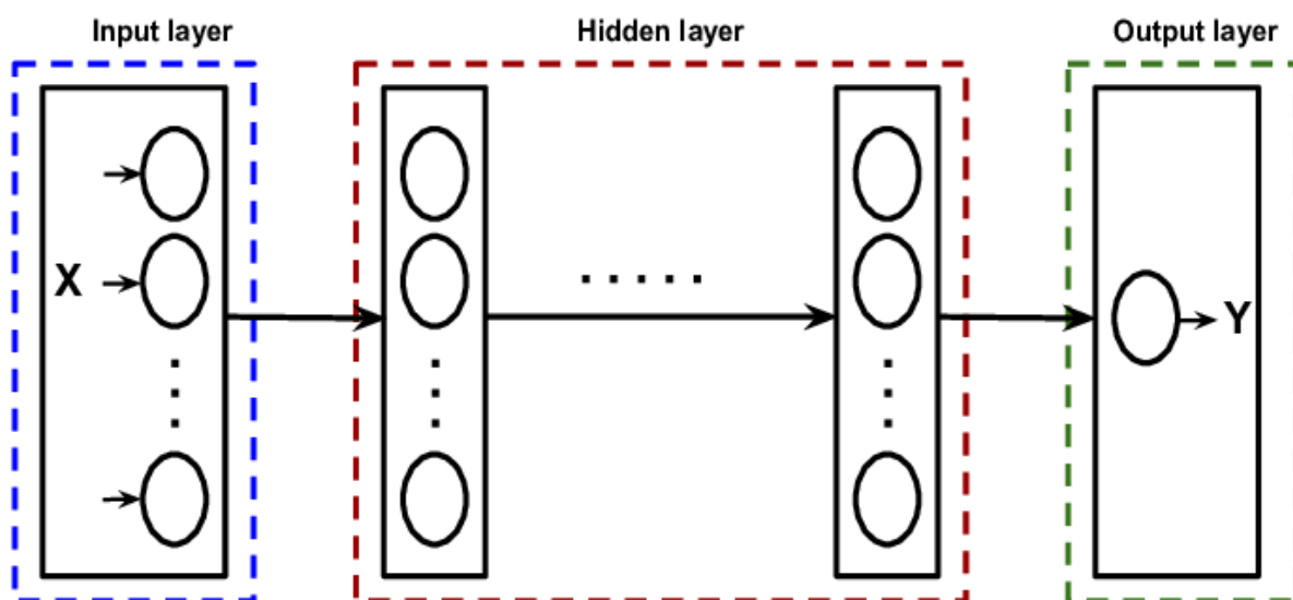
Figure 14 -MLP Regression
